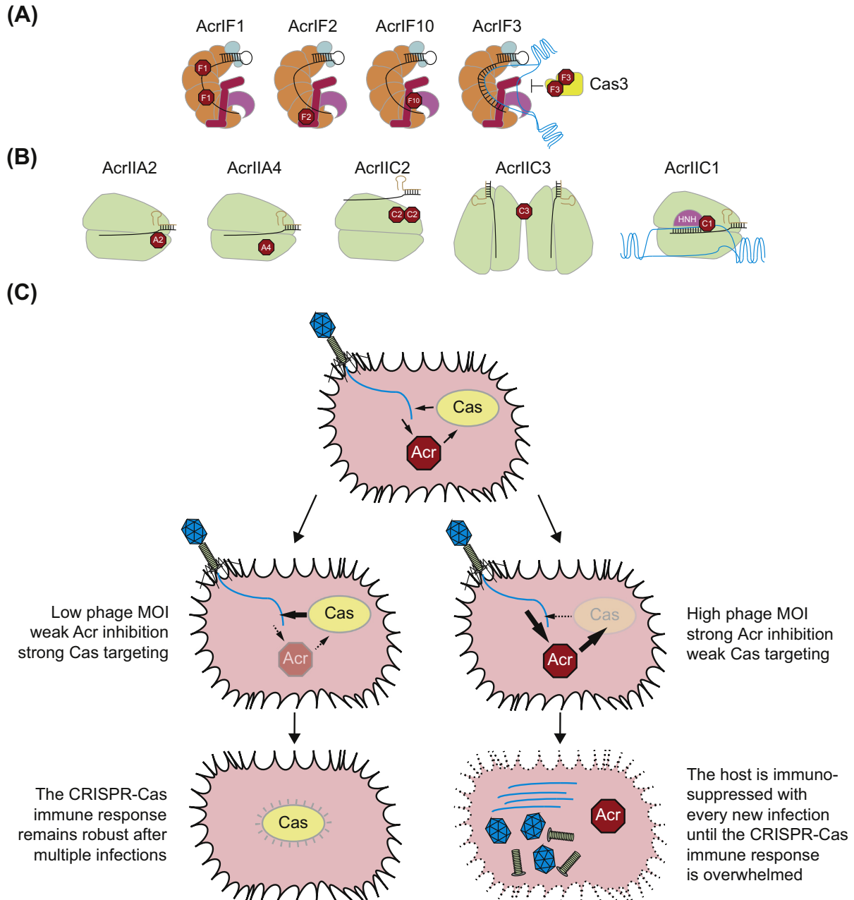
Figure 2. Mechanisms of Phage CRISPR Inhibitors. (A) CRISPR inhibitors of type I-F systems. The first class of inhibitors binds to the type I-F Cascade complex and prevent the binding of dsDNA. AcrIF1 binds the between Cas7f subunits at regular intervals, locking the complex in a formation that cannot bind dsDNA. AcrIF2 binds between the Cas7f and Cas8f subunits and AcrIF10 binds between Cas8f and Cas5f. Both inhibitors prevent the entry of DNA into the targeting complex. After the crRNA within Cascade (black line) has bound to its DNA target (blue line), the complex recruits Cas3, a DNase that degrades the target DNA. AcrIF3 forms a dimer that prevents recruitment of Cas3 to the targeting complex and blocks DNA entry into the Cas3 nucleolytic site. (B) CRISPR inhibitors of type II systems. AcrIIA2 and AcrIIA4 are inhibitors of the type II-A Cas9 nuclease. During target search Cas9 scans DNA for PAM, whose recognition is the first step in licensing DNA cleavage. AcrIIA2 and AcrIIA4 both bind the portion of Cas9 that recognizes the PAM, thus blocking DNA loading into the nuclease. AcrIIC2
