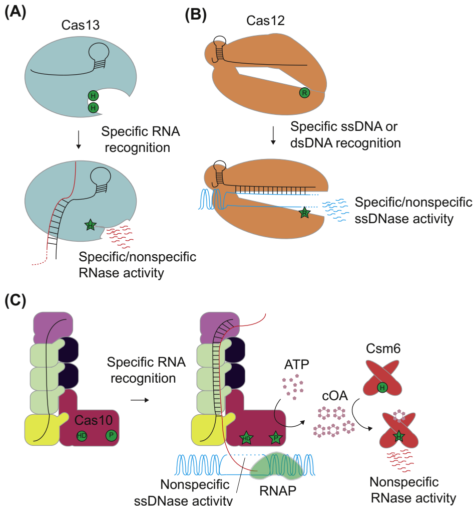
Figure 1. Collateral Nucleic Acid Degradation by Cas Nucleases and CRISPR Secondary Messenger Signaling. (A) RNA targeting by the type VI effector Cas13a. Cas13a possesses two HEPN domains (green circle, H). Binding of target RNA (red line) to the crRNA (black line) induces a conformational shift that brings the domains in close proximity to form an active HEPN site (green star). The active site then cleaves RNA in a sequence-independent manner. (B) Nucleic acid targeting by the prototypical type V effector protein, Cas12a. The RuvC domain (green circle, R) is responsible for the nucleolytic activity of Cas12a. Before target recognition, this domain is obscured by the Rec lobe. Upon binding of either dsDNA or ssDNA targets (blue lines) to the crRNA (black line), the effector undergoes a conformational shift that exposes and activates the RuvC domain (green star) to license cleavage of the target DNA and nonspecific cleavage of ssDNA. (C) Nucleic acid targeting and secondary messenger signaling by the type III-A CRISPR-Cas system. Upon recognition of a target transcript (red line) to the crRNA (black line), the type III complex activates multiple effector functions. The HD domain of the Cas10 subunit (green circle, H) is able to nonspecifically cleave ssDNA (blue line) from the transcription bubble. The Palm domain of Cas10 (green circle, P) is also activated and converts ATP into four or six member rings of cOA. cOA then acts as a secondary messenger and activates Csm6 by binding to its CARF (CRISPR-Associated Rossman Fold) domain causing activation of the HEPN domain (green circle, inactive, or green star, active; H), unleashing nonspecific RNA cleavage. Additionally, not depicted, a subunit of the type III complex, Csm3, is a specific RNase that cleaves the bound transcript. Abbreviations: cOA, cyclic oligoadenylate; CRISPR, clustered regularly interspaced short palindromic repeats; crRNA, CRISPR RNA; dsDNA, double-stranded DNA; HEPN, higher eukaryotes and prokaryotes nucleotide-binding; RNAP, RNA polymerase; ssDNA, single-stranded DNA.
