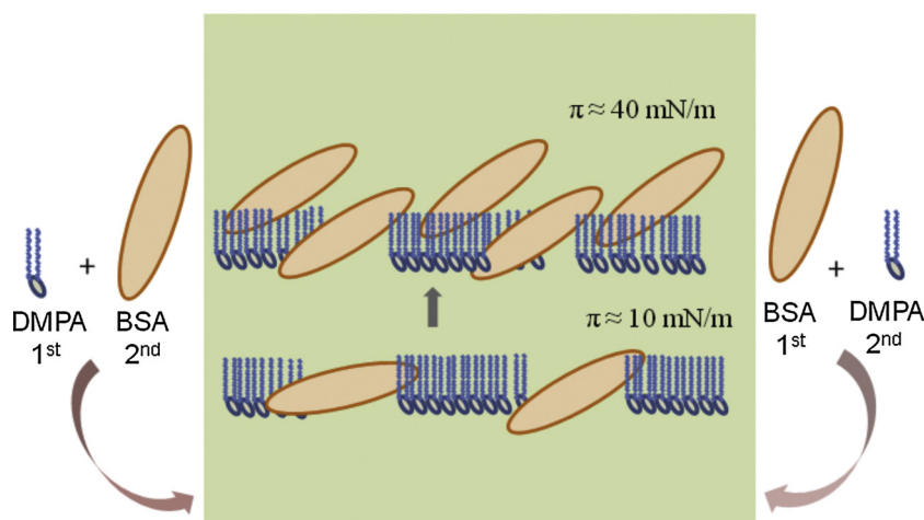
Fig. 8. Schematic representation of the structural modifications of the protein-lipid mixed films for lower (10 mN/m) and higher (40 mN/m) surface pressure at a particular subphase pH for two different spreading conditions, i.e., for B/D and D/B conditions. Nearly the same structural and morphological information are obtained for both the BSA-DMPA and DMPA-BSA mixed film.
