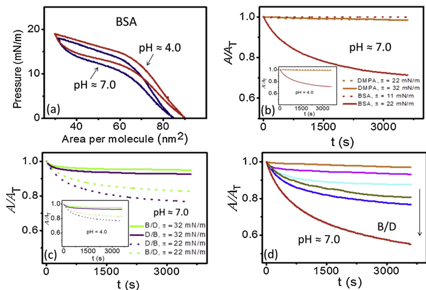
Fig. 3. (a) Compression-decompression isotherm cycles of BSA at pH \approx 4.0 (red) and \approx 7.0 (blue) respectively. (b) Stability curves (A-t) of the pure BSA, DMPA and mixed films (c) at lower (22 mN/m) and higher (32 mN/m) constant target pressures ( \pi_T ) at pH \approx 7.0. The insets show the same at pH \approx 4.0. (d) Stability for different ratios of BSA:DMPA mixed films are shown at pH \approx 7.0. Colours indicates the respective ratios of BSA:DMPA mixed films: red (150:0), blue (120:30), dark yellow (90:60), cyan (75:75), magenta (30:120) and orange (0:150), i.e., the corresponding BSA mole fractions ( X_B ) are 1.0, 68.7 \times 10^{-3} , 27.9 \times 10^{-3} , 17.7 \times 10^{-3} , 4.1 \times 10^{-3} and 0.0 respectively.
