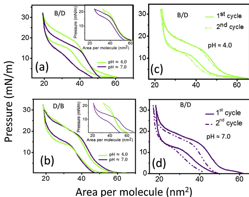
Fig. 2. Compression-decompression isotherm cycles of BSA and DMPA mixture (a) B/D and (b) D/B films at pH \approx 4.0 (green) and 7.0 (purple) at higher surface pressure (32 mN/m). The insets illustrate the corresponding isotherm cycles for lower surface pressure (22 mN/m). The consecutive two cycles of \pi -A isotherm in the B/D condition is shown for pH \approx 4.0 (c) and 7.0 (d) respectively.
