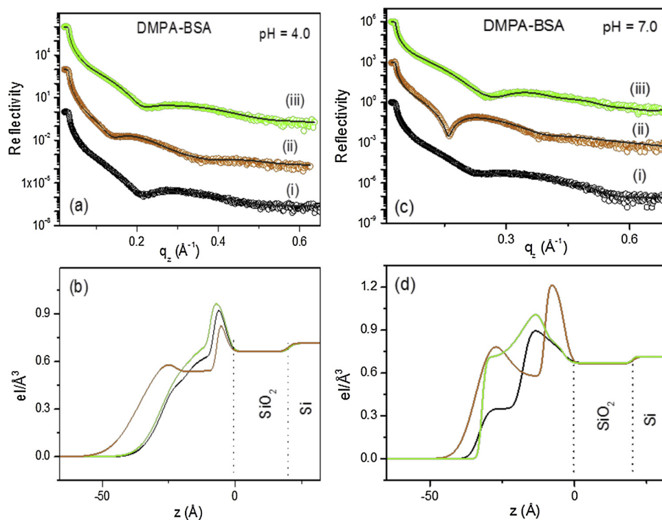
Fig. 6. X-ray reflectivity data (circle) and the corresponding fitted curves (solid line) obtained from the DMPA-BSA mixed films at (i) 10 mN/m and (ii) 40 mN/m during first compression, and again at (iii) 10 mN/m during second compression at (a) \text{pH} \approx 4.0 and (c) \text{pH} \approx 7.0 . (b) and (d): corresponding electron density profiles extracted from the fitting of the reflectivity data.
