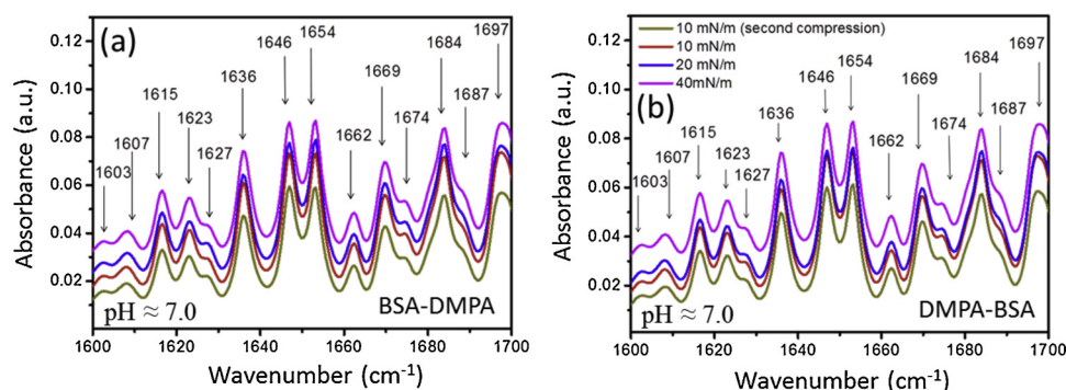
Fig. 5. ATR-FTIR spectra of Amide-I region obtained from (a) BSA-DMPA and (b) DMPA-BSA mixed films at \text{pH} \approx 7.0 for different pressure conditions, i.e., during first compression at pressure 10 mN/m (red), 20 mN/m (blue), 40 mN/m (magenta) and again at 10 mN/m (dark yellow) during second compression. Arrows indicate the corresponding peak positions.
