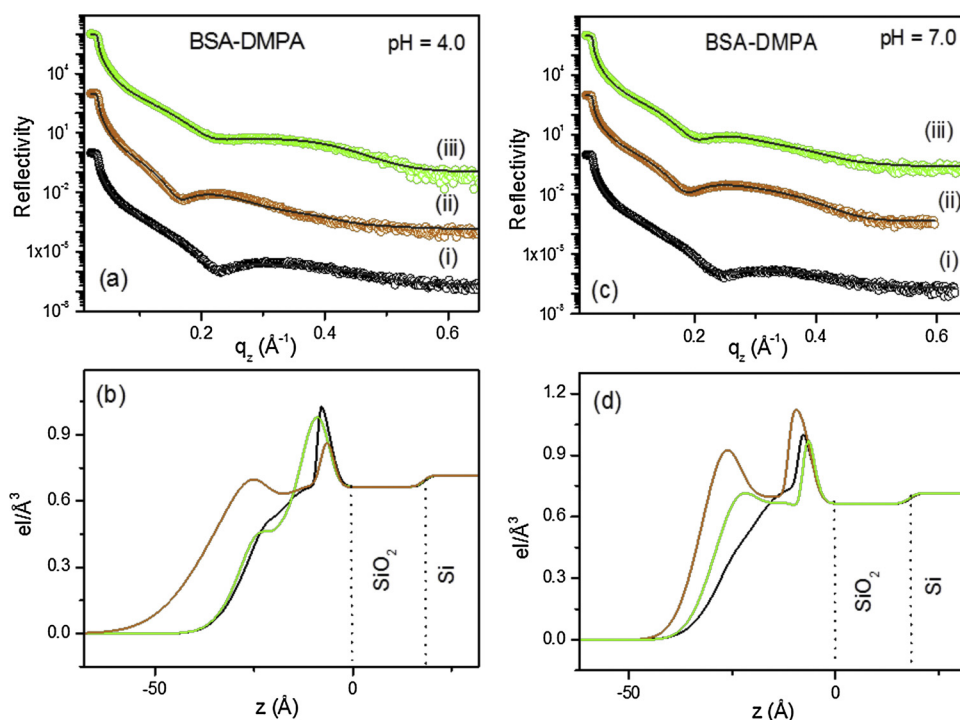
Fig. 7. X-ray reflectivity data (circle) and the corresponding fitted curves (solid line) obtained from the BSA-DMPA mixed films at (i) 10 mN/m and (ii) 40 mN/m during first compression, and again at (iii) 10 mN/m during second compression at (a) pH \approx 4.0 and (c) pH \approx 7.0. (b) and (d): corresponding electron density profiles extracted from the fitting of the reflectivity data.
