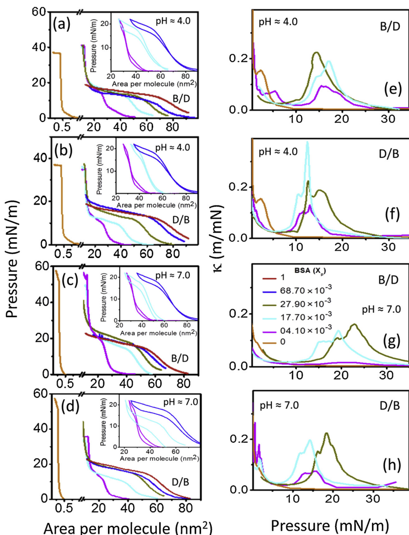
Fig. 1. Left Column: Surface pressure - mean molecular area ( \pi - A ) isotherms of BSA-DMPA mixed monolayer at two different subphase pH values, i.e., at \text{pH} \approx 4.0 (a–b) where figure (a) depicts B/D combinational order whereas figure (b) shows D/B order, and at \text{pH} \approx 7.0 where figure (c) and (d) stands for B/D and D/B combinational order respectively. Six colours represent six different ratios of BSA:DMPA mixed films: red (150:0), blue (120:30), dark yellow (90:60), cyan (75:75), magenta (30:120), orange (0:150). The corresponding BSA mole fractions ( X_p ) are 1.0 , 68.7 \times 10^{-3} , 27.9 \times 10^{-3} , 17.7 \times 10^{-3} , 4.1 \times 10^{-3} and 0.0 respectively. Inset: corresponding compression-decompression isotherm cycles of mixed films. Right Column (e–h) shows variation of isothermal compressibility ( \kappa ) with monolayer surface pressure ( \pi ) corresponding to their left counterparts of \pi - A isotherms.
