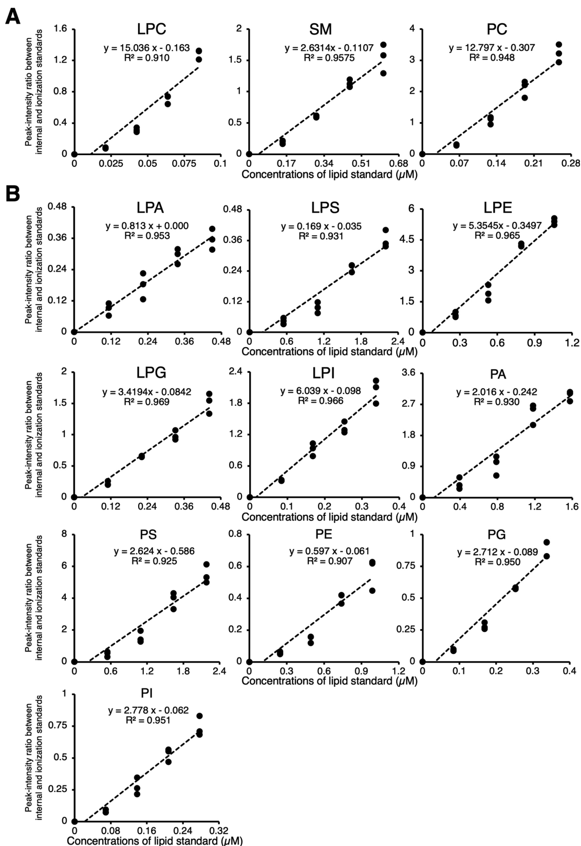
Fig. 4. Standard curves from quantitative MALDI analysis with internal STDs. The data shown in A and B were collected in the positive and negative modes, respectively. Coefficient of determination ( R^2 ) was calculated from the curve and evaluated to investigate the reliability of MALDI-TOF/MS for the quantitative analysis. Strong linear correlations were revealed between the normalized intensity and concentration of each lipid subclass, with R^2 values ranging from 0.907 to 0.969.
