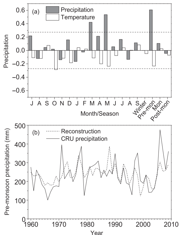
Fig. 2. Pre-monsoon precipitation signals recorded by the regional chronology. (a) Correlations between the regional chronology and monthly/seasonal temperature and precipitation; (b) comparison between the reconstructed and the CRU gridded precipitation in the pre-monsoon season.
