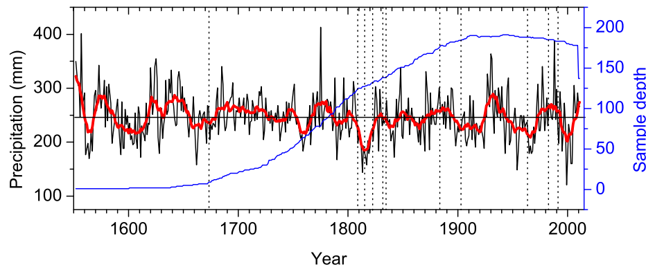
Fig. 3. Tree-ring based pre-monsoon precipitation reconstruction in this study. The years for 11 large tropical volcanic eruptions after 1650 [12] are indicated by dotted vertical lines.
