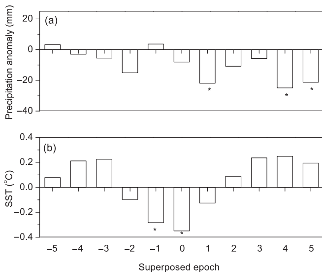
Fig. 4. Coupling between dry conditions, large tropical volcanic eruptions and cold SST. (a) Superposed epoch analysis between pre-monsoon precipitation events derived from a regional Himalayan tree-ring chronology and 11 tropical volcanic eruptions (1673, 1809, 1815, 1822, 1831, 1835, 1883, 1902, 1963, 1982 and 1991) selected by Fischer et al. [12] since 1650; (b) Superposed epoch analysis between dry years in the central Himalayas and tropical eastern Pacific SST [13]. Dry conditions since the early 20th century occurred in years and in the year before with significant cold SST; * shows significance at P < 0.05 .
