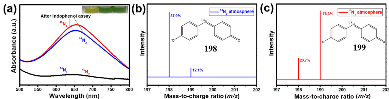
Fig. 5. The mass spectra of the indophenol prepared and UV-Vis absorption spectra from different atmosphere. (a) UV-Vis absorption spectra of the solutions from the nitrogen fixation reaction with ^{14}\text{N}_2 or ^{15}\text{N}_2 gas followed by the indophenol assay. Photos show the color change of the ^{14}\text{N}_2 and ^{15}\text{N}_2 solutions by the indophenol assay. MS spectra of derived indophenol solutions from (b) ^{14}\text{N}_2 and (c) ^{15}\text{N}_2 .
