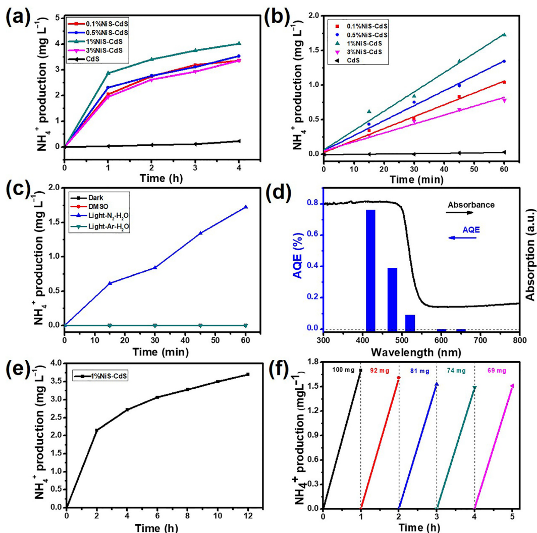
Fig. 4. Photocatalytic performance of the photocatalysts. (a) \text{NH}_4^+ production changes with the reaction time under full spectrum light irradiation. (b) \text{NH}_4^+ production changes with the reaction time under the visible light irradiation ( \lambda > 420 nm) within 1 h. (c) \text{NH}_4^+ production under different conditions (darkness, DMSO as solvent and water + light + N 2 or Ar) and exposure to visible light. (d) Apparent quantum efficiency (AQE) of NiS/CdS under visible light with different band pass filters (420, 475, 520, 600 and 650 nm). (e) \text{NH}_4^+ production changes with the reaction time under visible light irradiation ( \lambda > 420 nm) for 12 h. (f) Recycling experiment of NiS/CdS for five continuous cycles under visible light irradiation. The catalyst amounts were 100, 92, 81, 74 and 69 mg, respectively. The reaction dispersion concentration was maintained at 1 mg mL -1 for the five cycles.
