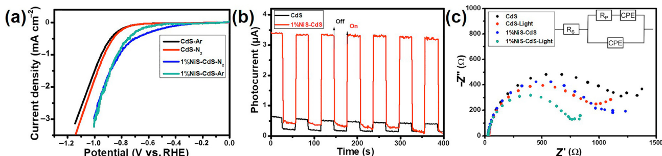
Fig. 3. Electrochemical performance of the photocatalysts. (a) Linear sweep voltammetry of CdS and NiS under an Ar and N_2 saturated solution. (b) Transient photocurrent of CdS and NiS/CdS. (c) Electrochemical impedance spectroscopy of CdS and NiS/CdS under light irradiation and dark conditions.
