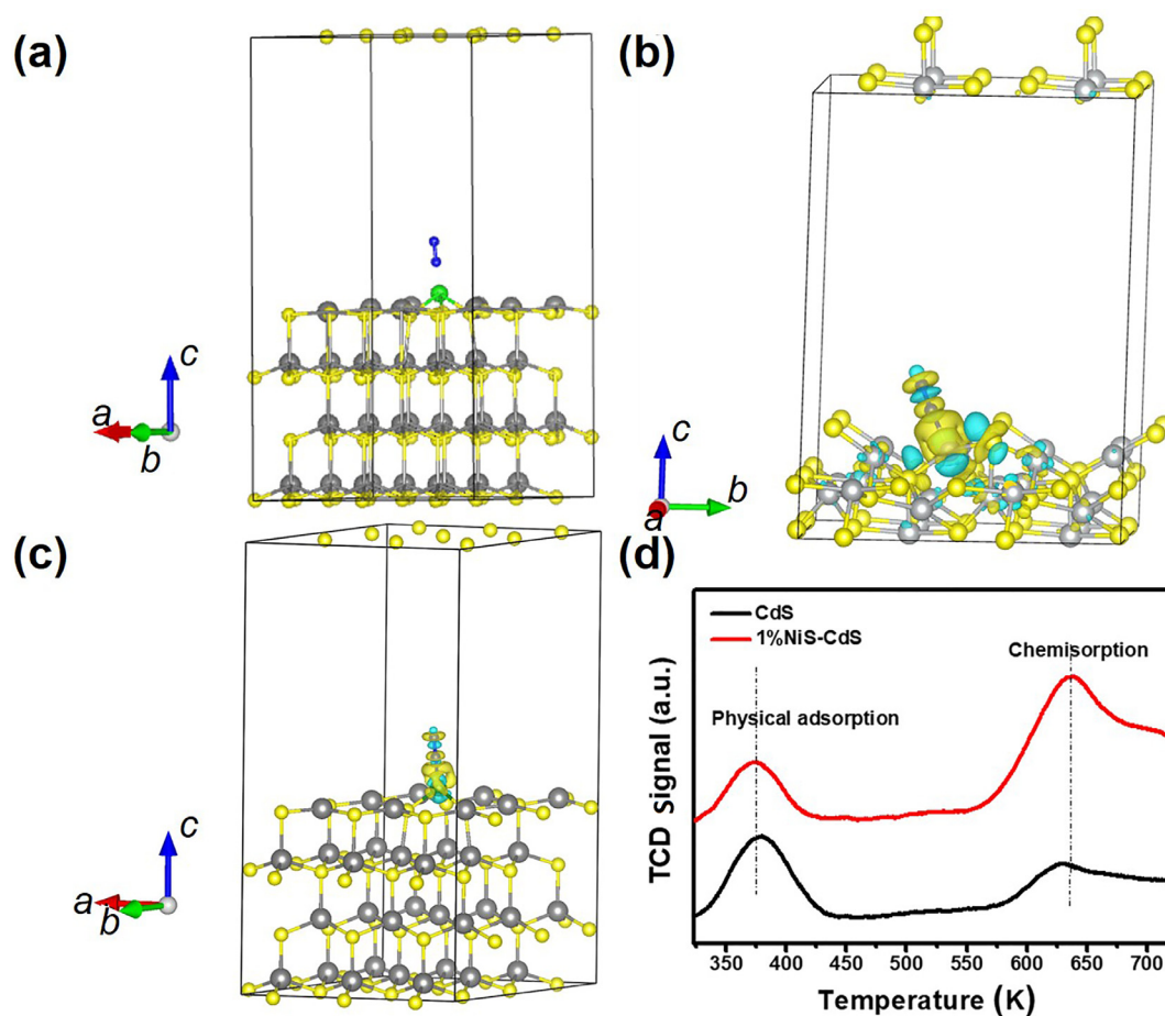
Fig. 2. N 2 adsorption on CdS and NiS/CdS nanorods. The theoretical adsorption energy of N 2 molecules on the CdS (002) surface (a), NiS (211) surface (b) and Ni doped CdS (002) surface (c). (d) Temperature programmed desorption (TPD) curves of N 2 on CdS and NiS/CdS.
