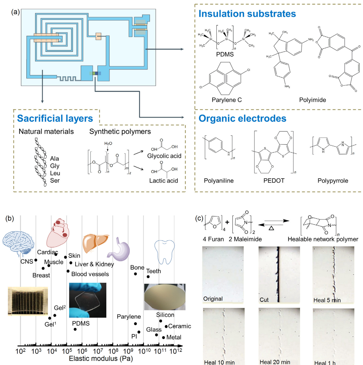
Fig. 2. (Color online) Polymers for soft interface and functionalization. (a) Different components with different polymers of a flexible bioelectronic device. (b) Logarithmic plot on the comparison of elastic moduli for various biological tissues and materials. (c) The realization of self-healing function by the use of self-healing polymer. Reprinted with permission from Refs. [4] and [34], Copyright 2017 Nature Publishing Group and 2013 Wiley-VCH Verlag.
