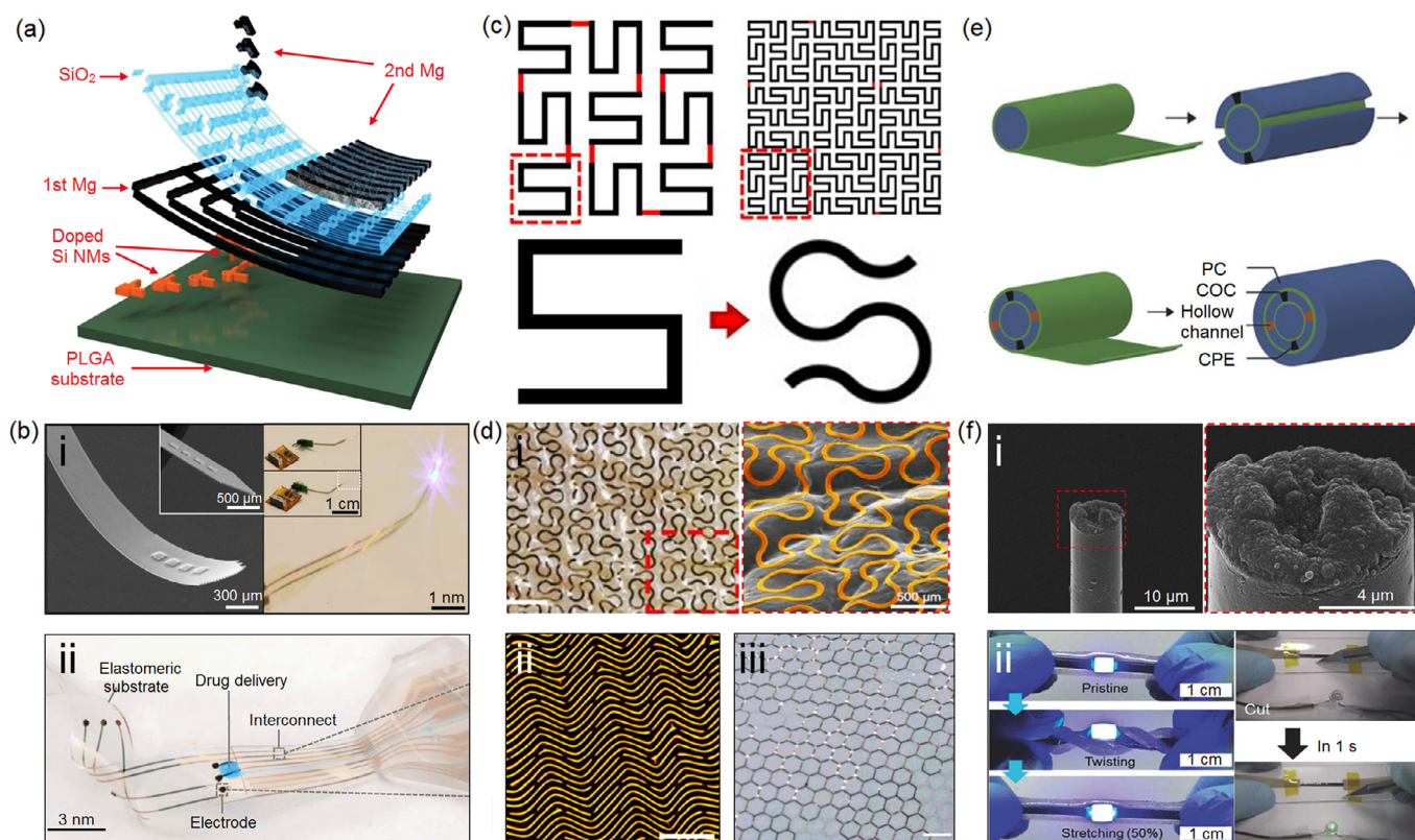
Fig. 3. (Color online) Structure design of flexible bioelectronic devices for dynamically mechanical stability. (a), (b) Structure and demonstration of typical planar compliant bioelectronic devices, respectively. (c), (d) Structure and demonstration of stretchable bioelectronic devices, respectively. (e), (f) Structure and demonstration of cable-like bioelectronic devices, respectively. Reprinted with permission from Refs. [6,2,37–40,46,7] and [25], Copyright Wiley-VCH Verlag, Science Publishing Group, Nature Publishing Group and American Chemical Society.
