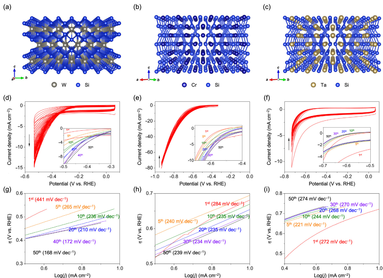
Fig. 3. (Color online) Electrochemical behaviour of other silicides. (a–c) Crystal structure of WSi 2 , CrSi 2 , and TaSi 2 . (d–f) CVs and (g–i) the corresponding Tafel plots of WSi 2 , CrSi 2 , and TaSi 2 in 1 mol L -1 KOH. Insets show the corresponding enlarged views in (d–f).
