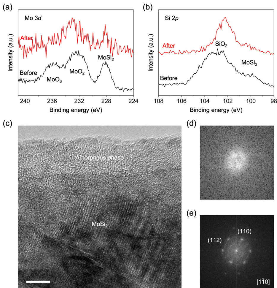
Fig. 4. (Color online) Surface evolution of MoSi 2 . (a) Mo 3d and (b) Si 2p XPS spectra of MoSi 2 before and after CV activation in 1 mol L -1 KOH. (c) HRTEM image of MoSi 2 after activation along the [1–10] zone axis, with a low-contrast thin layer indicating the silicon oxide shell. (d) Fourier transform images of the amorphous shell and (e) MoSi 2 core. Scale bar is 5 nm.
