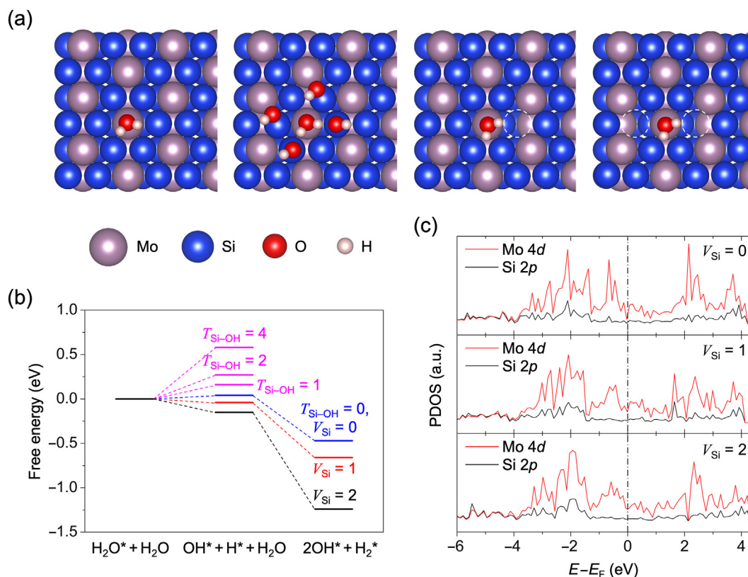
Fig. 5. (Color online) Density functional theory calculations of hydrogen evolution on MoSi 2 . (a) Optimized geometry of pristine MoSi 2 (1 1 0) surface with adsorbed H 2 O and other MoSi 2 (110) surfaces with adsorbed H 2 O and OH groups/Si vacancies. (b) Free energy versus the reaction coordinate of alkaline HER for different MoSi 2 surfaces. (c) Calculated projected density of states (PDOS) plots of Mo 4d and Si 2p orbitals for pristine MoSi 2 and other MoSi 2 surfaces with Si vacancies.
