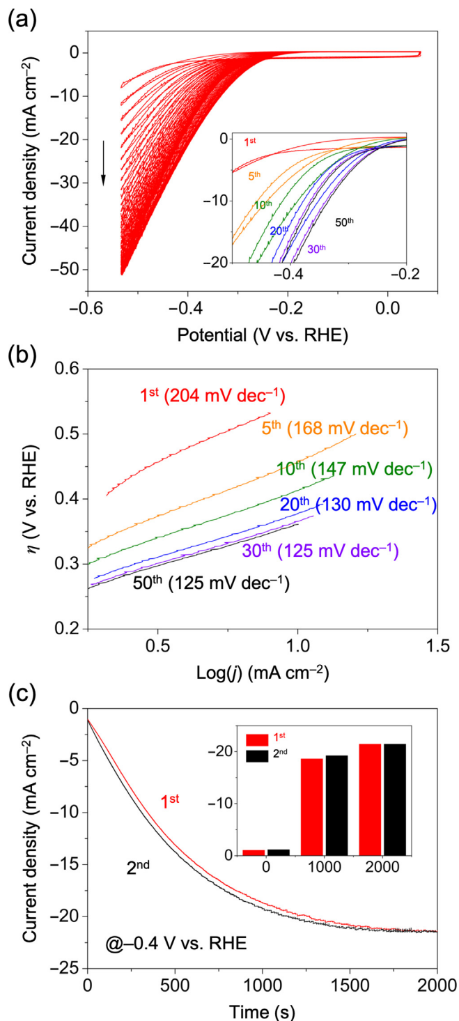
Fig. 2. (Color online) Electrochemical behaviour of MoSi 2 . (a) CVs and (b) the corresponding Tafel plots of MoSi 2 in 1 mol L -1 KOH. (c) Chronoamperometric i - t curves of MoSi 2 at -0.4 V vs. RHE for different sequences in 1 mol L -1 KOH. Insets show the corresponding enlarged view and histogram of current densities in (a) and (c), respectively.
