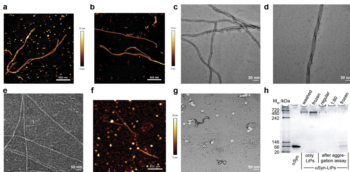
Fig. 5. Sample properties at the end of the aggregation assays. AFM images of αSyn fibrils grown in the presence of POPG αSyn-LiPs, before centrifugation (a) and after removal of the supernatant (b). c + d) EM image of αSyn fibrils grown in the presence of POPG αSyn-LiPs before centrifugation (condition 64x in Fig. 4c). e) EM image of αSyn fibrillar structures grown in the presence of POPG αSyn-LiPs that did not lead to sizable ThT signal increase (condition 4x in Fig. 4c). f + g) AFM and EM image of POPG αSyn-LiPs control samples at the end of the aggregation assays (without addition of excess of monomeric αSyn, Fig. 4b). d) Native PAGE of monomeric αSyn as well as αSyn-LiPs in indicated conditions (washed refers to high-salt washed; frozen = non-washed, flash frozen and stored at -20^{\circ}\text{C} ; regular = non-washed, non-frozen; 1:80 = preparation with high salt and adapted molar ratio of αSyn to lipids of 1:80). Note that amount of monomers added in aggregation assays is identical to amount loaded in the free αSyn control (first lane).
