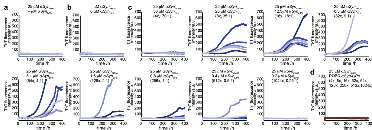
Fig. 4. αSyn-LiPs can induce primary nucleation. a–d) ThT aggregation assays under quiescent conditions. Under these conditions neither aggregation of αSyn in the absence of αSyn-LiPs (a) nor of αSyn-LiPs on their own (b) is observed. Each plot contains data of five replications of the indicated condition. c) Variation of αSyn-LiP level in the presence of constant monomeric αSyn starting concentrations. In addition to concentration of monomeric αSyn, also the concentration of αSyn in LiPs is provided for each plot. Numbers in parentheses refer to estimated excess of monomeric αSyn over αSyn-LiP particles (assuming an average composition of 8 αSyn per LiP (Eichmann et al., 2016)). In addition, the respective molar ratios of lipids to added monomeric αSyn are given in (c) but using POPC αSyn-LiPs (all 45 curves are shown in one plot).
