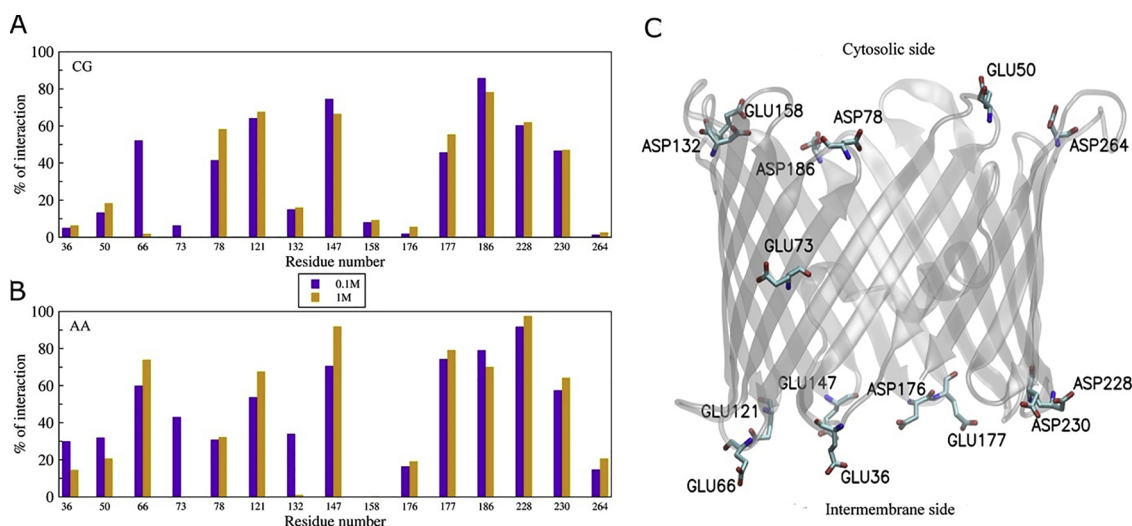
Fig. 7. Percentage of interactions formed between the lipid head amine group of POPE and side chain of VDAC individual acidic residues at 0.1 M (purple bar) and 1 M (orange bar) KCl in CG (A) and atomistic (AA) (B) MD simulations. C. Locations of acidic residues forming interactions with the POPE head group featuring a percentage higher than about 10% in CG MD and atomistic MD. The only acidic residue which is not located at the rim of the channel but nevertheless interacts with POPE head group is E73. This residue is located in the middle of \beta -strand 4 and points towards the hydrophobic membrane environment in all determined 3D structures (C). The binding of dicyclohexylcarbodiimide, a chemical that covalently links acidic residues in a hydrophobic environment, to E73 supports this unusual surrounding for an acidic residue (De Pinto et al., 1993).
