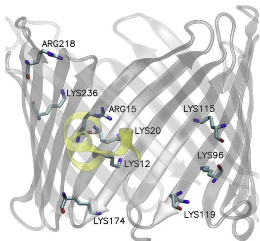
Fig. 1. Side view of the 3D structure of mVDAC1 (PDB ID: 3emn (Ujwal et al., 2008)) shown as a white transparent cartoon. The N-terminal helix is highlighted in yellow. The basic residues found in MD simulations to be important for ion translocation are also depicted as atom-type colored sticks and labeled.
