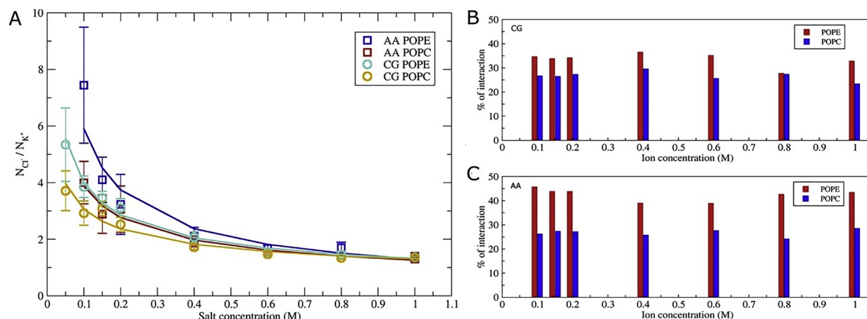
Fig. 6. The VDAC selectivity is affected by the nature of the lipid. (A) The selectivity measured as the N_{Cl^-}/N_{K^+} ratio as a function of the bulk KCl concentration for VDAC embedded in either POPE or POPC bilayer (CG MD/POPE (cyan spheres), CG MD/POPC (orange spheres), atomistic MD/POPE (blue square), atomistic MD/POPC (red square)). For each data point the standard error is shown as a bar. The fitting procedure is described in Fig. 2. (B, C) Percentage of interactions formed between the lipid head amine group of POPE (red bar) or POPC (blue bar) and the side chain of all VDAC acidic residues as a function of salt concentration in CG (B) and atomistic (AA) (C) MD simulations.
