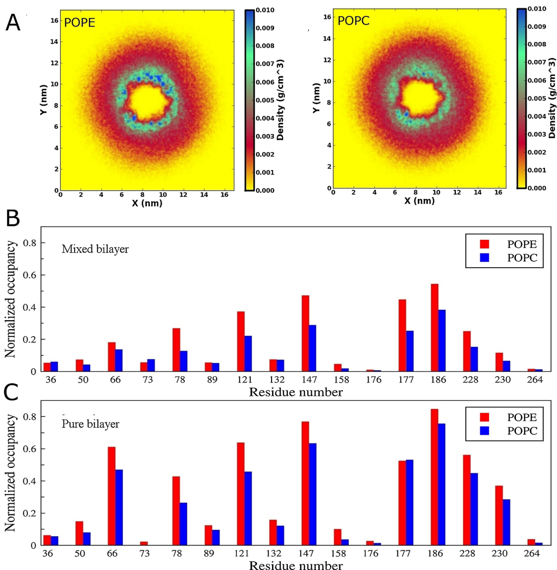
Fig. 8. Interaction of VDAC acidic residues with lipid molecules. (A) 2-D projections of the spatial density function (SDF) of POPE and POPC amine head group around the intermembrane opening region of VDAC. The SDFs were calculated for a Z-slice 10 Å wide containing the intermembrane space head group region in the POPE/POPC mixture CG simulations. A density color scale is shown on the right. (B–C) Normalized maximum occupancy calculated around each VDAC acidic residue side chain, averaged over CG simulations in (B) POPC/POPE mixed bilayer and (C) pure POPE and pure POPC bilayers.
