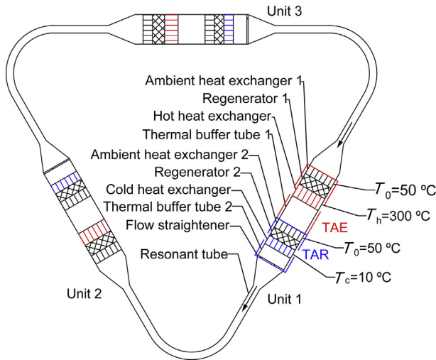
Fig. 1. The three-unit direct-coupling HD-TAR.
