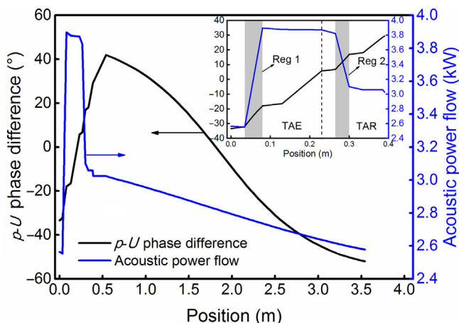
Fig. 2. The axial distributions of the p - U phase difference and the acoustic power flow in one unit.
