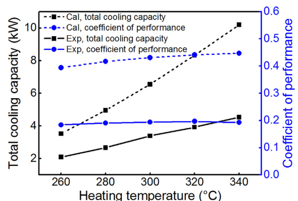
Fig. 3. Experimental and calculated results, total cooling capacity and coefficient of performance at 10 °C.
