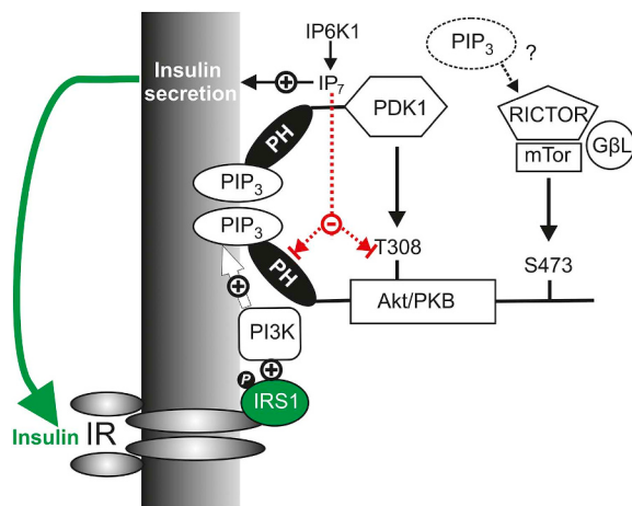
Fig. 2. Model of possible regulation of Akt/PKB by inositol pyrophosphates in \beta -cells. Proposed model illustrates that although IP_7 may inhibit Akt/PKB in pancreatic \beta -cells, its dominant effect could be to activate Akt/PKB, through the insulin feedback loop.
