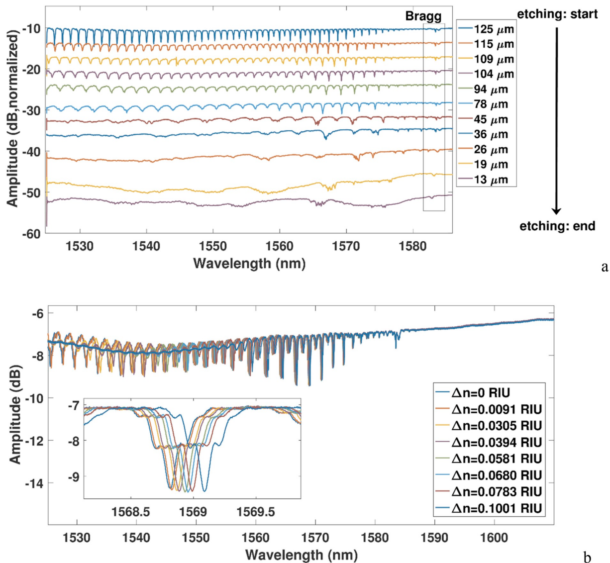
Fig. 3. (a) Reflection spectra throughout the HF etching of the TFBG; (b) Spectral change of the eTFBG ( d = 94 \mu\text{m} ) for different sucrose concentrations; inset: zoom on the modes where the analysis was carried out.
