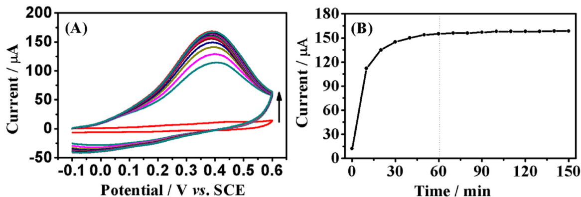
Fig. 2. Optimization of the experimental conditions. (A) CVs of hairpin DNA/MCH/tDNA/PBIB modified gold electrode in eATRP mixture. Scans were taken every ten minutes. Scan rate: 1.0 \text{ V s}^{-1} . The concentration of tDNA was 10 \text{ fM} . (B) The plot of peak current versus eATRP time.
