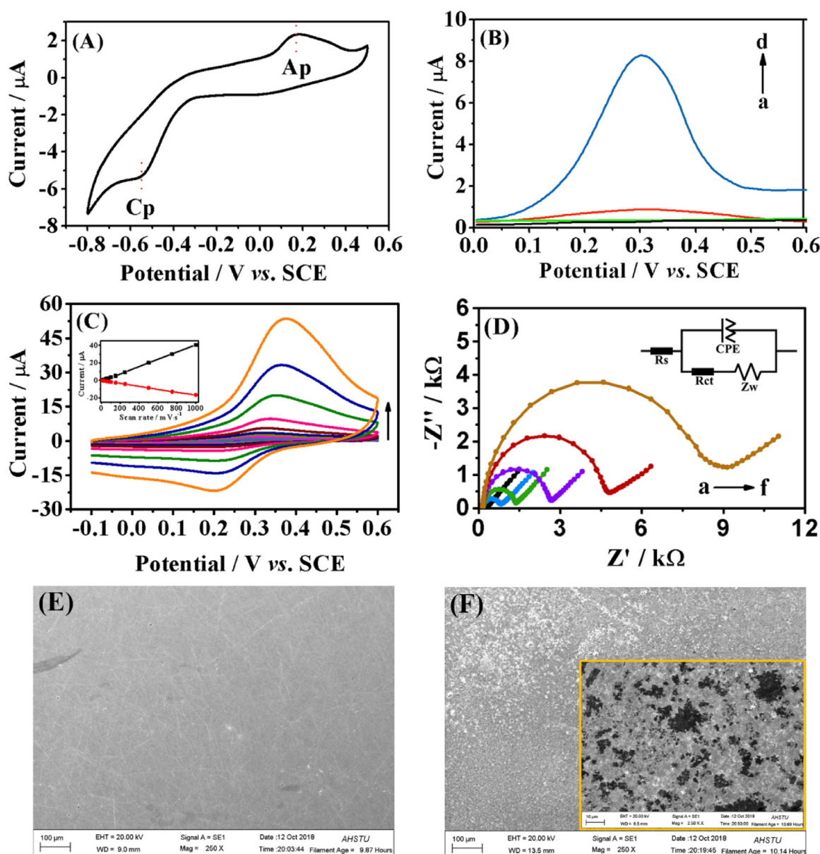
Fig. 1. (A) CVs of the hairpin DNA /MCH/tDNA/PBIB -modified gold electrodes in the FMMA-free eATRP mixture. The concentration of tDNA was 10 fM. Scan rate: 0.1 \text{ V s}^{-1} . (B) SWV curves of bare gold electrode(a), hairpin DNA/MCH/PBIB/FMMAgold electrode (b), hairpin DNA/MCH/tDNA/ECgold electrode(c), and hairpin DNA/MCH/tDNA/PBIB/FMMA modified gold electrode (d) in \text{LiClO}_4 . (C) the CVs of hairpin DNA/MCH/tDNA/PBIB/FMMA modified gold electrode at different scan rate ranging from 10 to 1000 \text{mV s}^{-1} . Inset: The relationship between oxidation (black line) and reduction (red line) peak currents and scan rates in 1.0 M \text{LiClO}_4 ; (D) The Nyquist plots of the bare gold electrode (a), hairpin DNA modified gold electrode (b), hairpin DNA/MCH modified gold electrode (c), hairpin DNA/MCH/tDNA modified gold electrode (d), hairpin DNA/MCH/tDNA/PBIB modified gold electrode (e) and hairpin DNA/MCH/tDNA/PBIB/FMMA modified gold electrode (f). EISs were obtained in 0.1 M \text{KNO}_3 aqueous solution containing 5 mM \text{K}_3[\text{Fe}(\text{CN})_6]/\text{K}_4[\text{Fe}(\text{CN})_6] . (E) The SEM image of hairpin DNA/MCH/tDNA/PBIB/gold electrode. (F) The SEM image of the polymer-grafted gold electrode (hairpin DNA/MCH/tDNA/PBIB/FMMA modified gold electrode). Inset is the SEM image of the polymer-grafted gold electrode with high resolution.
