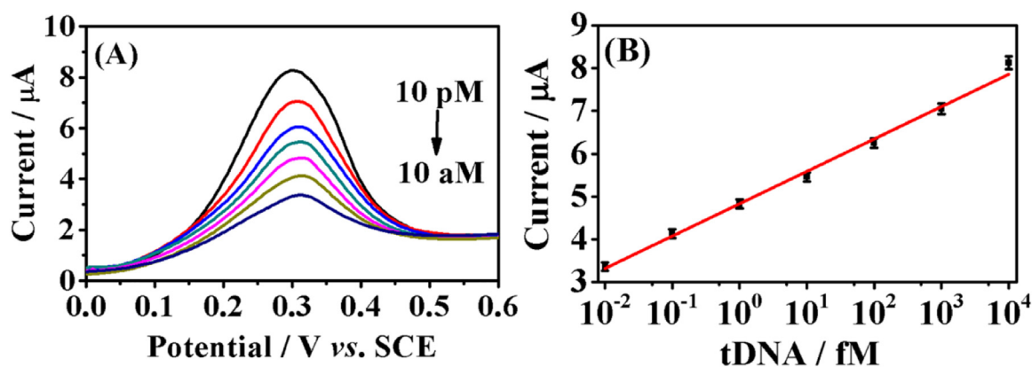
Fig. 3. (A) The SWV responses of the biosensor in the presence of different concentrations of T-DNA. The concentrations of T-DNA over the range of 10 aM to 10 pM. (B) Corresponding calibration curve. The error bars were obtained based on six repetitive experiments.
