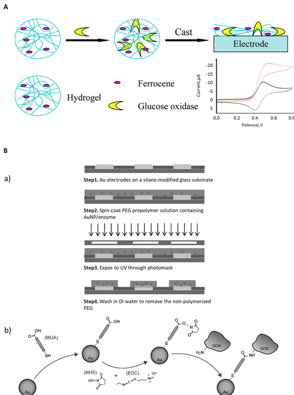
Fig. 4. Enzyme immobilization approaches in 3D biosensors. A) GOx entrapment in a hydrogel made of ferrocene and phenylalanine (Qu et al., 2014). B) Similar micropatterned manufacture approach, with patterning nanocomposite hydrogels, incorporating AuNPs, previously conjugated with of GOx on Au electrode arrays. (a) Overall micropatterned process; (b) Covalently binding chemistry of GOx enzymes to AuNPs (Pedrosa et al., 2011). The incorporation of GOx conjugated AuNPs allowed 100-fold improvement on glucose sensitivity. Figures reproduced with permission from ACS publications and Wiley.
