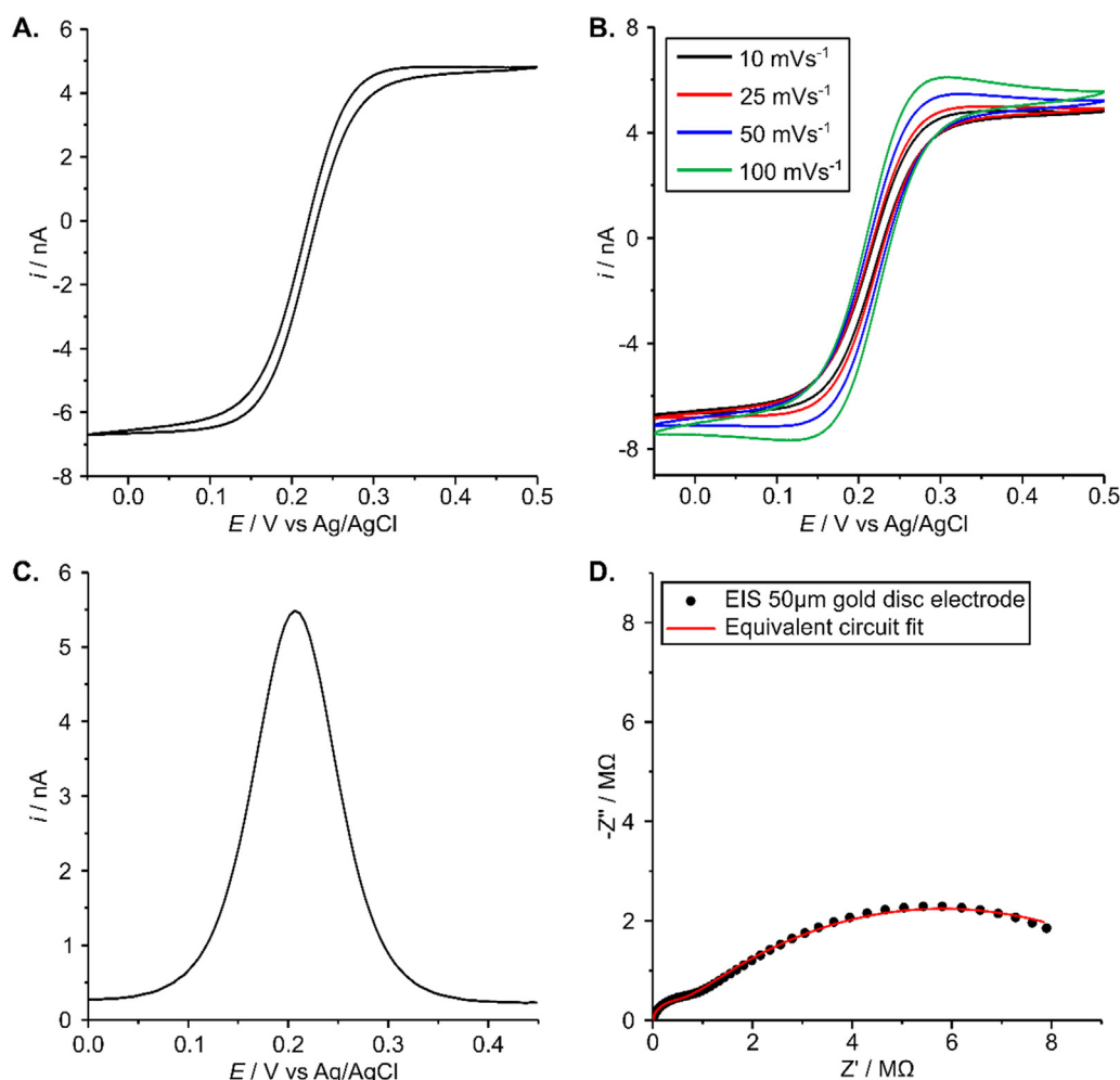
Fig. 3. Electrochemical characterisation of an r = 25 \mu\text{m} disc electrode. (A) Cyclic voltammetry (CV) at 10 \text{ mVs}^{-1} . (B) Cyclic voltammetry over a range of sweep rates ( 10, 25, 50 and 100 \text{ mVs}^{-1} ). (C) Differential pulse voltammetry (DPV). (D) Electrochemical impedance spectroscopy (EIS) recorded at open circuit potential.
