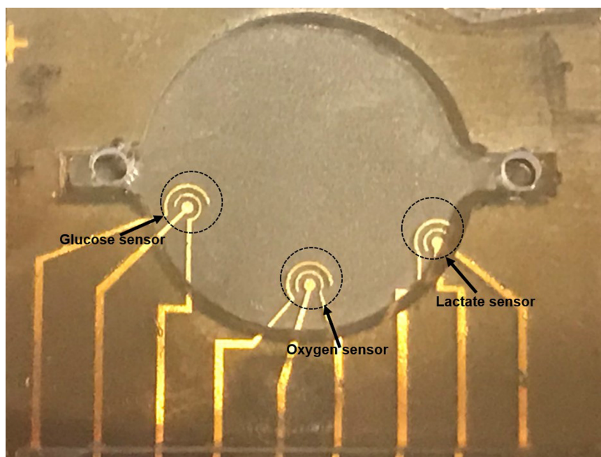
Fig. 1. Complete design with 3 mm thick SU8 micro-chamber covered by a glass lid.
