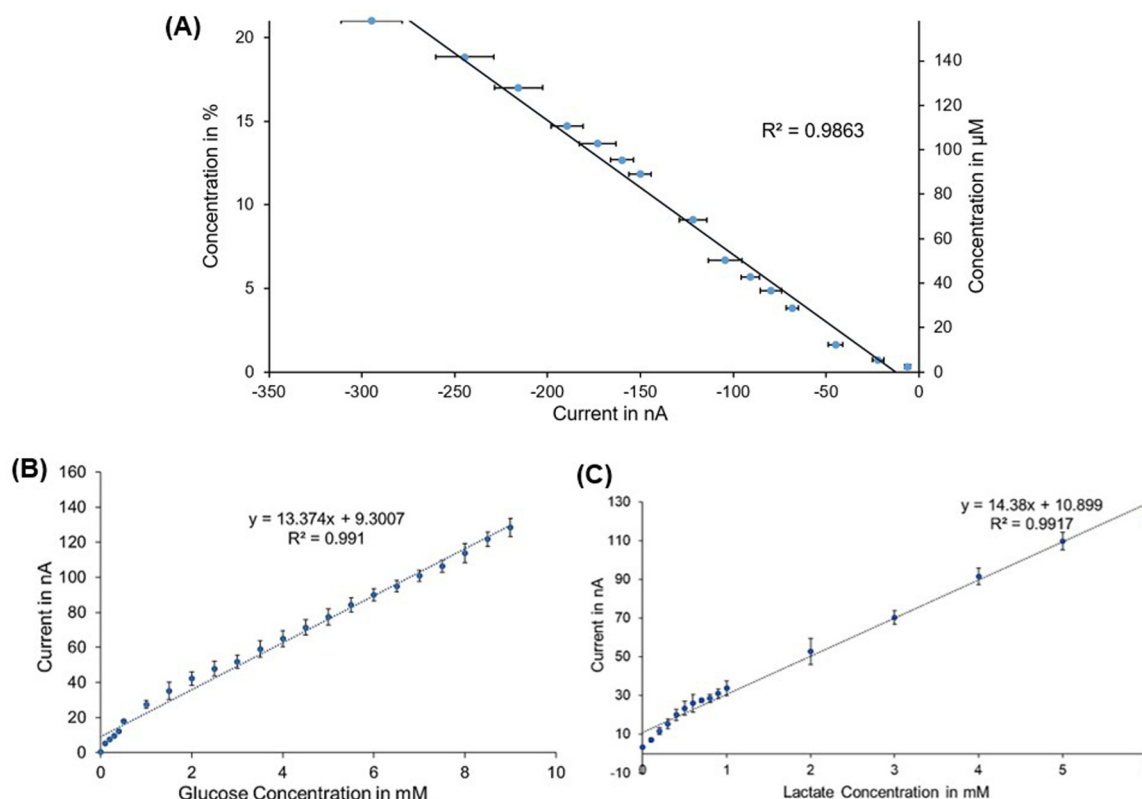
Fig. 2. (A) Oxygen sensor calibration curve: left y-axis represents concentration in %, right y-axis is concentration in \mu\text{M} . (B) Glucose sensor calibration curve. (C) Lactate sensor calibration curve. (Error bars in each curve are standard deviations (SD) between 6 data points).
