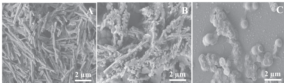
Fig. 1. The characteristic SEM images of MA-Cu nanorods in the (A) absence and the presence of (B) \text{Cl}^- ions, and (C) then GSH.
