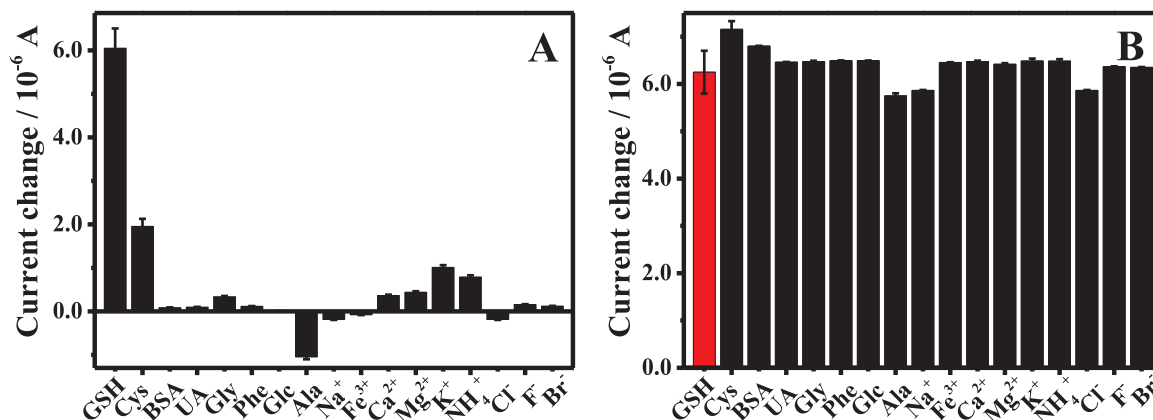
Fig. 3. Electrochemical LSV responses of the MA-Cu nanorods modified electrodes to (A) different interferences indicated alone, and (B) interferences mixed separately with GSH of same concentration (300.0 \mu\text{M} ).
