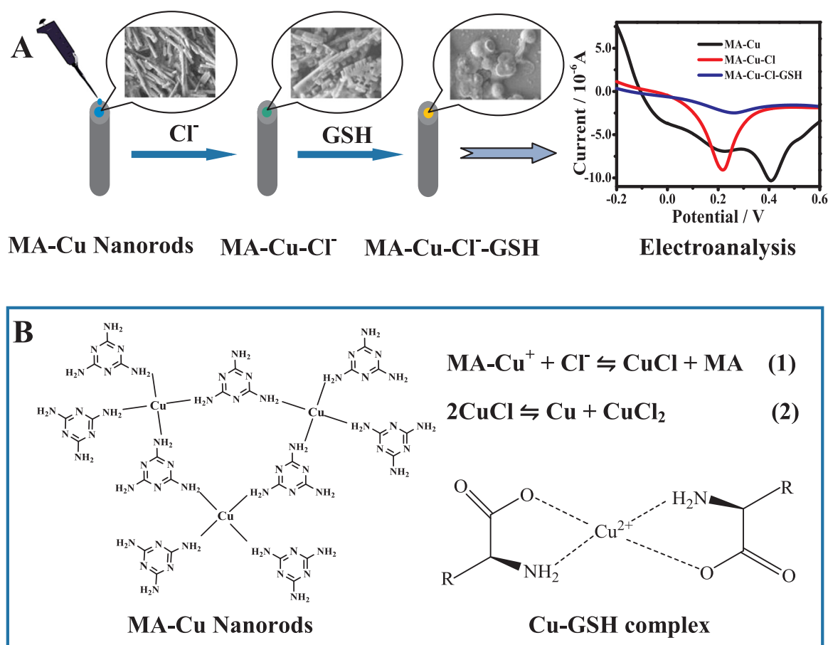
Scheme 1. Schematic illustration of (A) the step-by-step setup of the MA-Cu nanorods modified electrodes with the electrochemical responses to \text{Cl}^- ions and then GSH (top: SEM images of the resulting products); (B) the structural formula of MA-Cu nanorods prepared by the supermolecular self-assembly (left), in which the Cu-Cl reactions and Cu-GSH complex would undergo (right).
