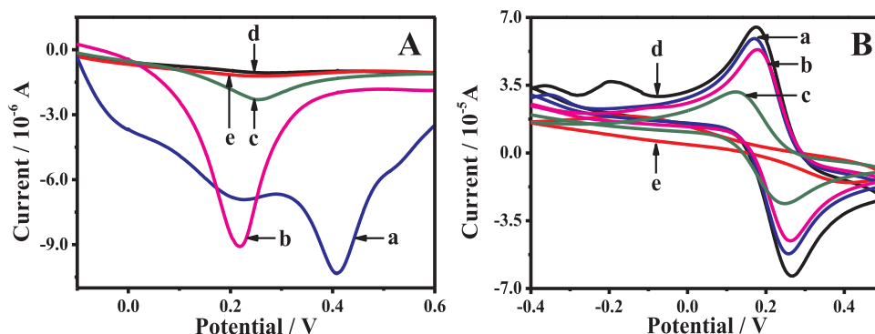
Fig. 2. (A) Characteristic electrochemical LSVs and (B) conductivity investigations with \text{K}_3[\text{Fe}(\text{SCN})_6] probes for the MA-Cu nanorods modified electrodes (a) before and (b) after adding \text{Cl}^- ions, and then (c) GSH, taking (d) the bare electrode and (e) the MA-modified electrodes as the controls.
