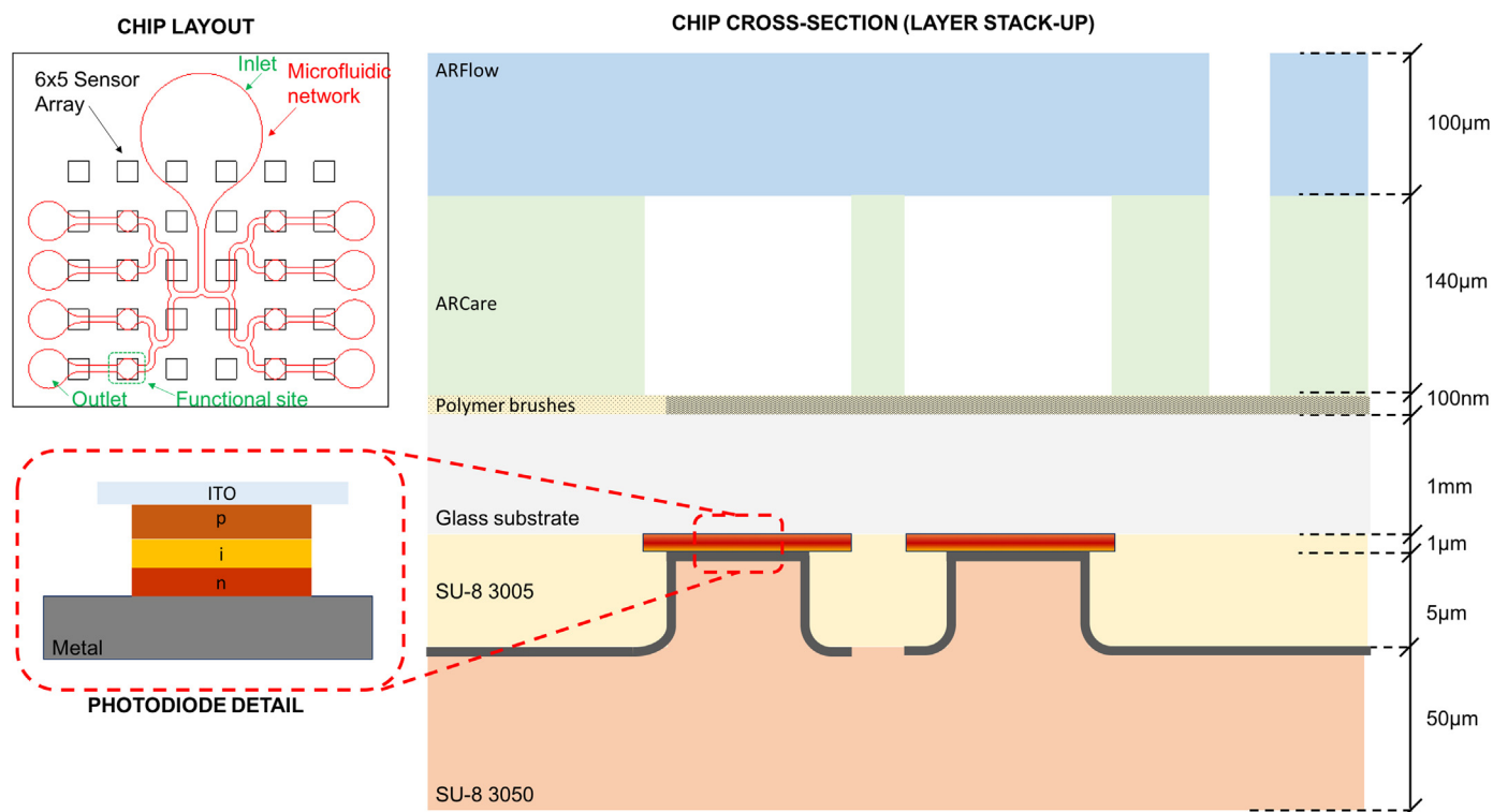
Fig. 1. Schematic view of the PLEIADES chip. Top-left: simplified chip layout view showing the position of the 30 photodiodes (squares) and the shape of the microfluidic network with one inlet and 8 identical branches, each having a functional site and an outlet. Right: cross-section of the chip (not to scale). The thickness of each layer is reported on the right. Bottom-left: detail of the thin-film a-Si:H p-i-n photodiode with transparent contact at the glass side to measure the CL signal coming from the opposite side of the glass.
