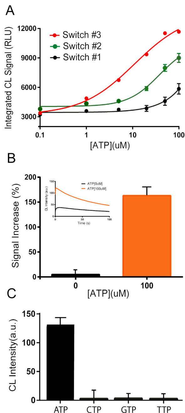
Fig. 5. : (A) chemiluminescence binding curves of DNA-nanoswitches variants (#1, #2, #3) in the presence of increasing ATP concentrations. (B) For nanoswitch #3 we observed an increase in activation of 160%. (C) The DNAszyme remains inactive when challenged with other non-specific targets. Incubation with 100 μM of different nucleoside triphosphates, for example CTP, GTP, TTP, does not produce any significant signal increase.
