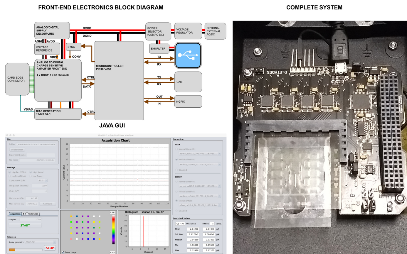
Fig. 2. Top-left: block diagram of the electronic front-end showing its main components and connections. Bottom-left: screenshot of the Java Graphical User Interface acquired during a test experiment. Right: picture of the whole system inside the black metallic shielding box with the PLEIADES chip attached to the card edge-connector. The PLEIADES front-end board has PC-104 format and has been designed according to electronics reliability guidelines.
