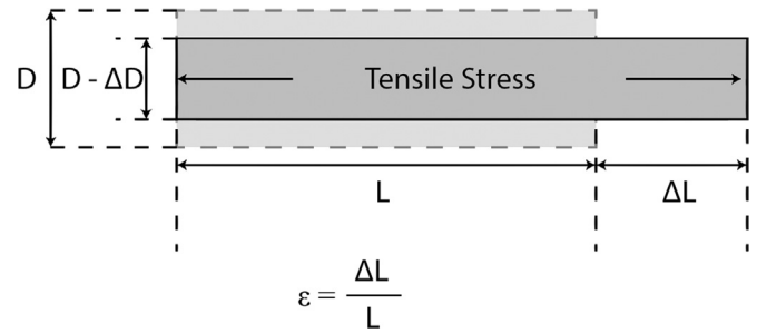
Fig. 1. Illustration of strain in materials.
