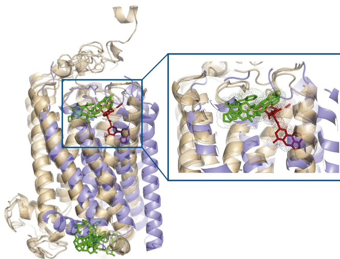
Fig. 3. Cartoon representation of molecular docking between receptors (in blue the 4IB4 template and in gold the corresponding target SRT-29) and ligand (ergotamine, in red). In green the ergotamine docking poses are shown for the predicted structure. (For interpretation of the references to colour in this figure legend, the reader is referred to the web version of this article.)
