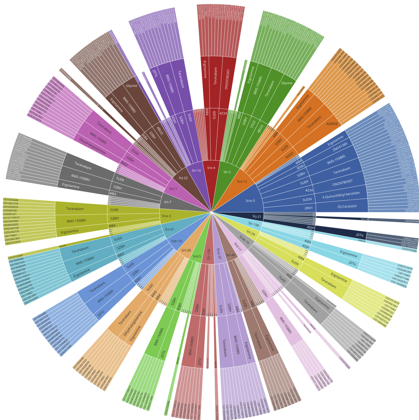
Fig. 2. For each GPCR of C. elegans the entire pipeline path is shown. Starting from the inner circle, the names of the 21 genes are indicated. Each of these is mapped on a larger circle where GPCR I-Tasser template proteins are indicated. Considering only GPCR template proteins in complex with a ligand, the third circle shows the names of the ligands associated with the template proteins. The outermost layer contains the names of the alternative ligands which are similar to the ligands selected in terms of physical-chemical characteristics.
