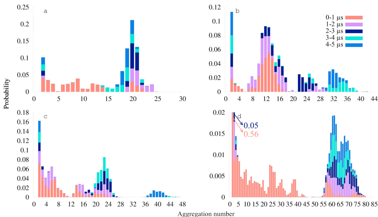
Fig. 3. The cumulative probability distributions of aggregation numbers as a function of time (block-averaged over 1 \mu s intervals) for systems A (Fasted-8000 nm 3 ), B (Fasted-16,000 nm 3 ), C (Fasted-20,000 nm 3 ), and D (Fed-16,000 nm 3 ). The regions including larger aggregation numbers in part (d) are omitted for clarity.
