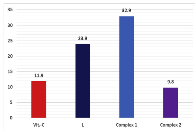
Fig. 4. IC_{50} values of L , 1 , 2 and Vit-C.
