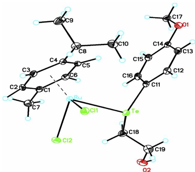
Fig. 2. Molecular structure of complex [\text{RuCl}_2(\text{p-cymene}) (\text{L})] ( 2 ).
