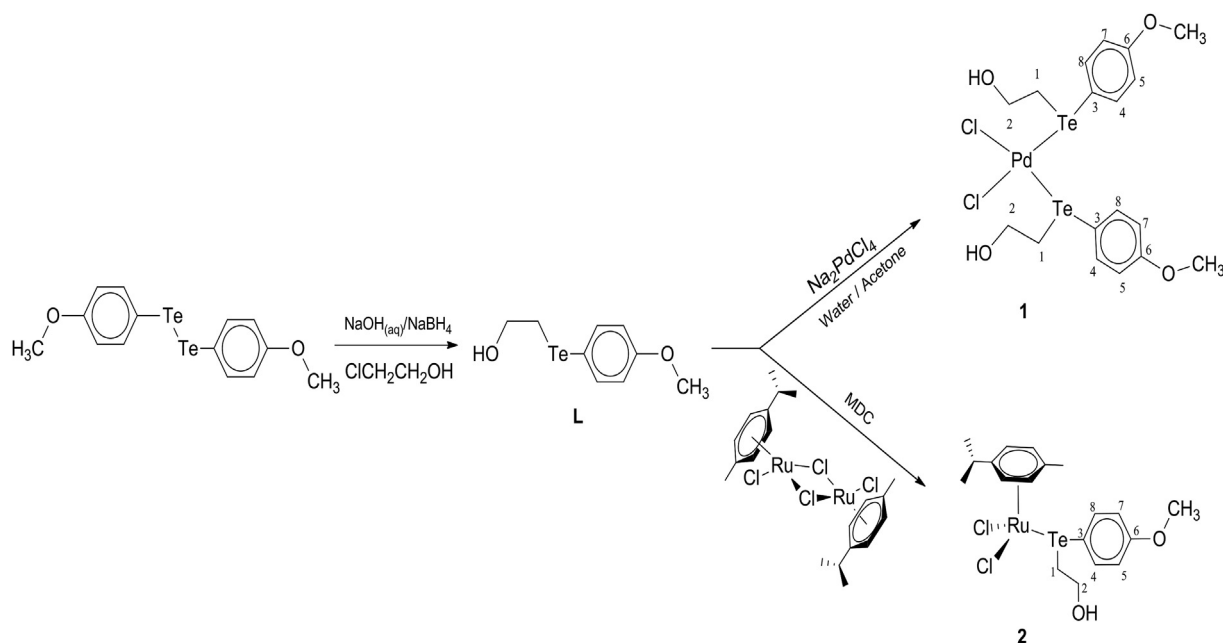
Scheme 1. Synthesis of ligand, L and its complexes, cis-[PdCl 2 (L) 2 ] ( 1 ), and [Ru(η 6 - p -cymene)Cl 2 (L)] ( 2 ).
