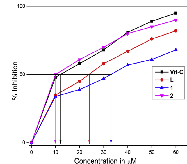
Fig. 3. Antioxidant activity as percentage inhibition of DPPH radicals against concentration of L , 1 , 2 and Vit-C.
