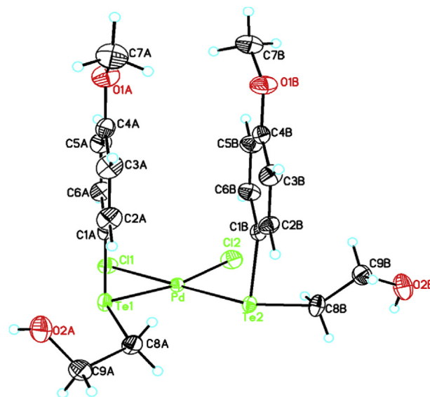
Fig. 1. (a) Molecular structure of complex cis -[PdCl 2 (L) 2 ] ( 1 ).
