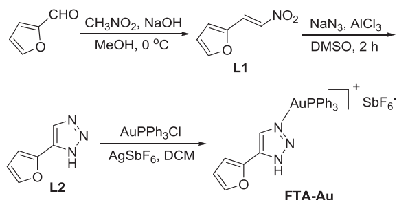
Scheme 2. Synthesis and X-ray of FTA-Au.
