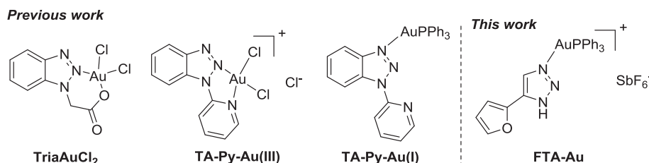
Scheme 1. Several gold complexes.
