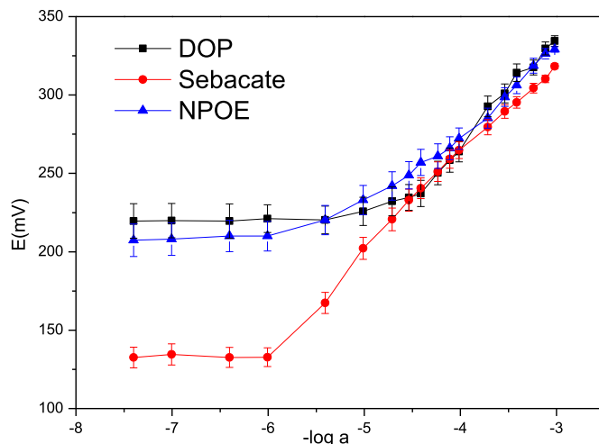
Fig. 3. ISE response: Potentiometric response of Sulfapyridine selective \mu SE with different plasticizers in the membrane.
