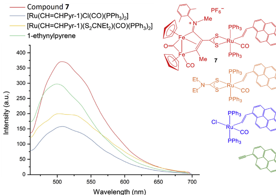
Fig. 1. Emission spectra of 7 , [\text{Ru}(\text{CH}=\text{CHPyr-1})(\text{S}_2\text{CNEt}_2)(\text{CO})(\text{PPh}_3)_2] , [\text{Ru}(\text{CH}=\text{CHPyr-1})\text{Cl}(\text{CO})(\text{PPh}_3)_2] and 1-ethynylpyrene ( \lambda_{\text{exc}} = 450 \text{ nm} ) in dichloromethane solution (100 \mu\text{M} ).
