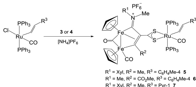
Scheme 2. Preparation of heterotrimetallic group 8 complexes 5 – 7 .
