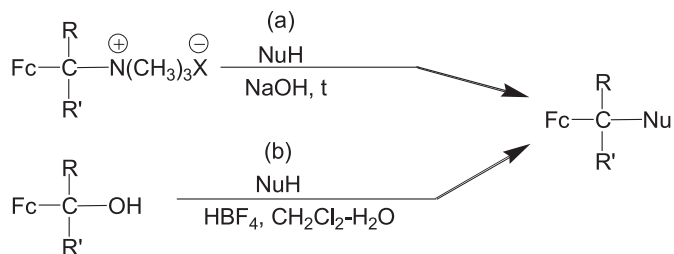
Scheme 1. \alpha -Ferrocenylalkylation reactions using \alpha -ferrocenylalkylammonium salts (a) or \alpha -ferrocenyl substituted alcohols (b) (Nu – nucleophile).
