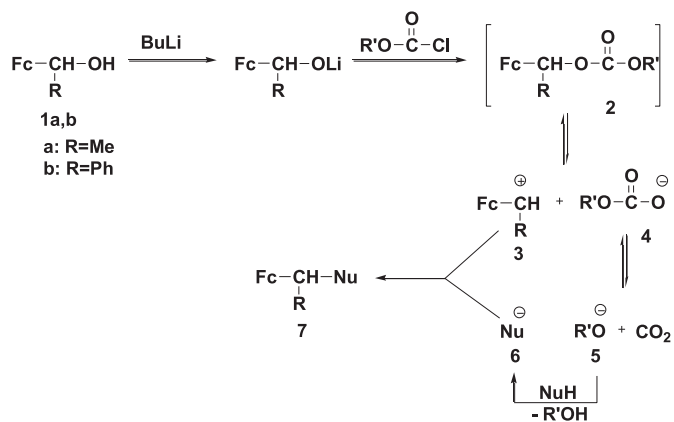
Scheme 2. \alpha -Ferrocenylalkylations with \alpha -ferrocenylalkyl carbonates 2 .
