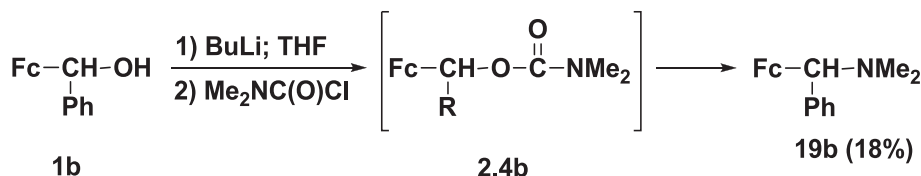
Scheme 8. Decomposition of carbamate 30b in the absence of an external nucleophile.
