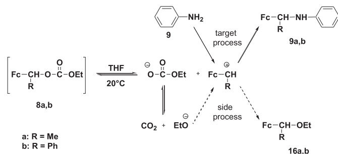
Scheme 3. The competitive target and side processes on the decomposition of FcCH(R)OC(O)OEt ( 8a,b ) in the presence of PhNH 2 ( 9 ).
