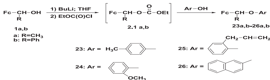
Scheme 4. \alpha -Ferrocenylalkylation of ArOH.
