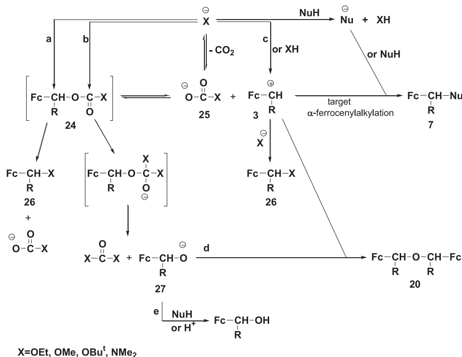
Scheme 7. \alpha -Ferrocenylalkylation of NuH with \text{FcCH(R)OC(O)X} and competitive side reactions.
