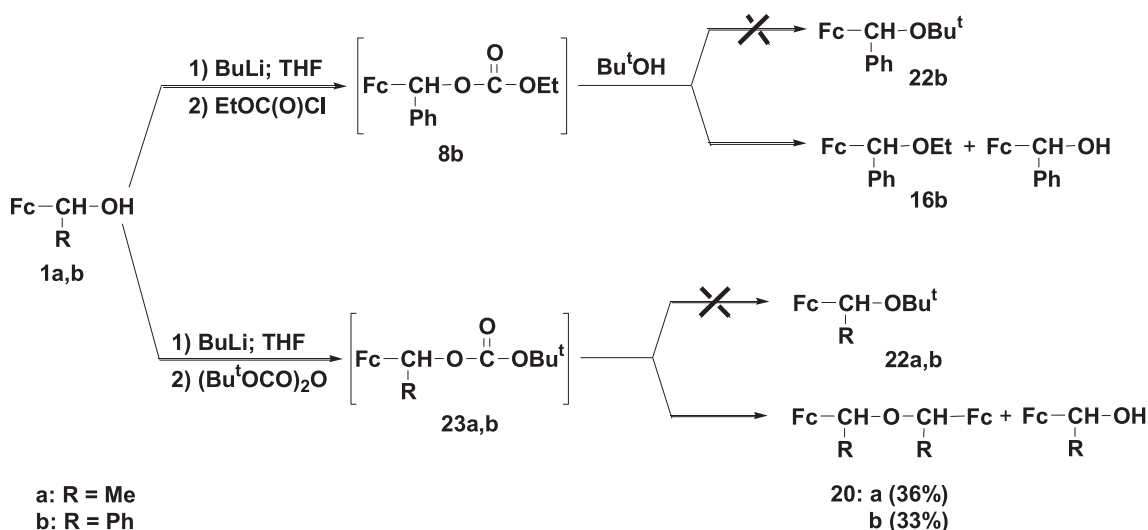
Scheme 6. The unsuccessful attempts to prepare \text{FcCH(R)O}^t\text{Bu}^t ( 22 ).
