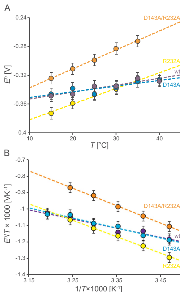
Fig. 3. Redox thermodynamics of the high-spin native form of KpDyP and the variants D143A, R232A, and D143A/R232A. (A) Temperature dependence of the reduction potential E^\circ . (B) Plot of E^\circ/T versus 1/T . KpDyP (violet), D143A (blue), R232A (yellow) and D143A/R232A (orange). The slopes of the plots yield the \Delta S^\circ_{rc}/F (A) and -\Delta H^\circ_{rc}/F (B), respectively. Solid lines are least-squares fits to the data points. All experiments were conducted in 150 mM phosphate buffer and 100 mM NaCl at pH 7.0. (For interpretation of the references to color in this figure legend, the reader is referred to the web version of this article.)
