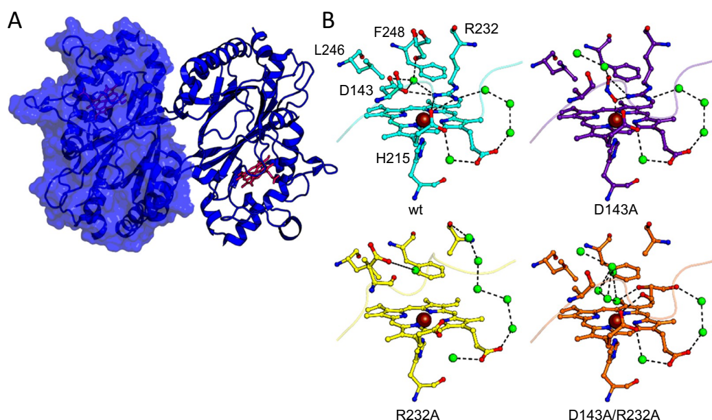
Fig. 1. Overall structure of dimeric wild-type dye-decolorizing peroxidase of Klebsiella pneumoniae (KpDyP) and active site structures of the variants D143A, R232A, and D143A/R232A.
