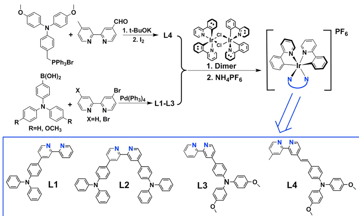
Scheme 1. Synthesis process of cyclometalated Ir III complexes.
