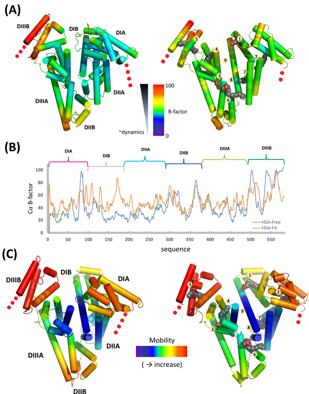
Fig. 3. Ligands affect HSA's dynamics: (A) The 3D crystal structures of HAS with colored C\alpha B-factors; left panel HSA-free (PDB ID: 1AO6) and right panel HSA-FA (PDB ID: 1E7H). (B) The plot depicting the differences along the HSA sequence for the HSA-free and HSA-FA together with the location of domains. (C) The approximation of the protein conformational dynamics done by the Gaussian Network Model algorithm [188] revealing the differences in molecular motions between the two structurally the most distant Human Serum Albumin crystal structures. The domain names and FA binding sites are marked as in (A).
