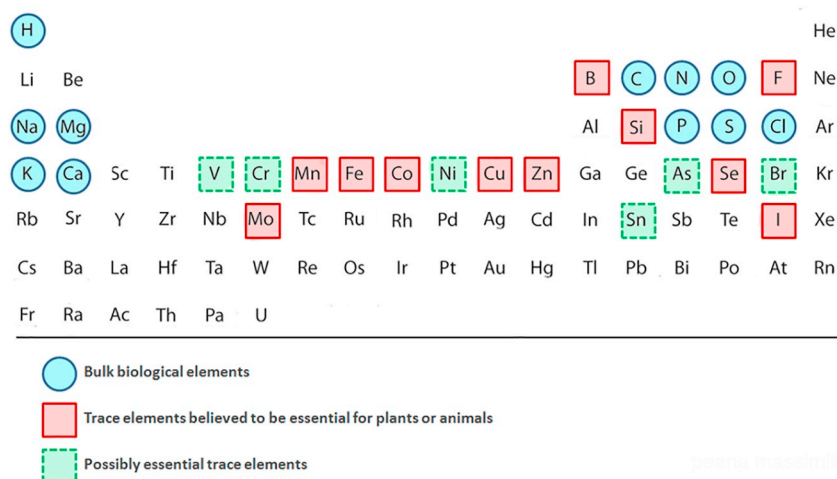
Fig. 1. The periodic table of the chemical elements required for life.
