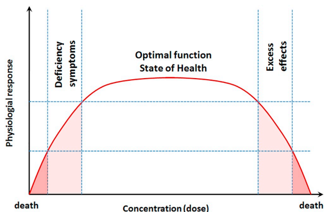
Fig. 2. Dose-response diagram for an essential element.
