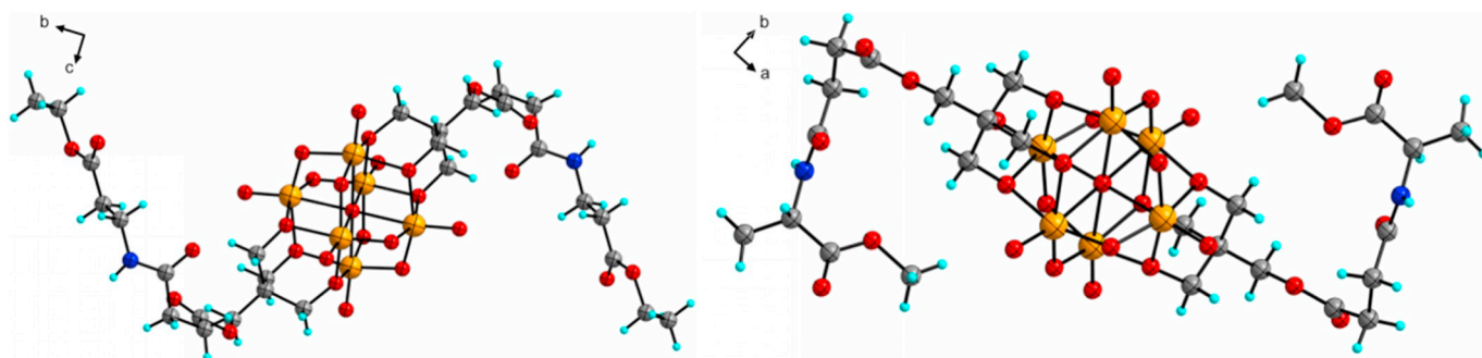
Fig. 1. ORTEP drawings of the anion structures of compounds 2 (left) and 3 (right). Red sphere: O; light blue sphere: H; grey sphere: C; blue sphere: N; orange sphere: V.
