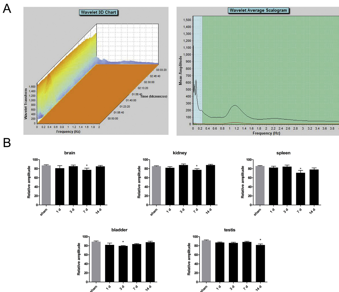
Fig. 1. Spectral analysis of endothelial factors. A, Corresponding vasomotor amplitude during the study period. B, Values of the relative amplitudes of the oscillatory LDF signal for endothelial factors. n = 6 in each group. * P < 0.05 compared with the sham group.
