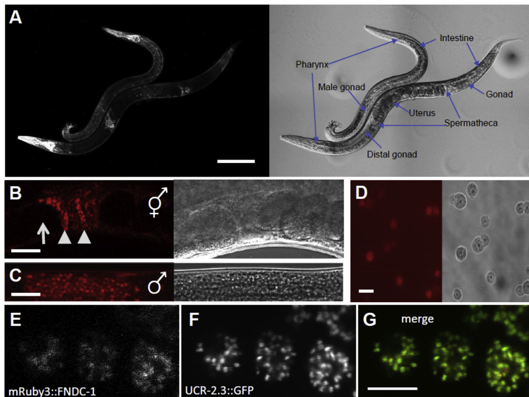
Fig. 1.. FNDC-1 is expressed in spermatids and targeted to mitochondria. mRuby3 red fluorescent protein sequence was inserted into the N-terminal genomic coding region of fndc-1 using CRISPR-Cas9 editing and HDR. Images in panels A–D contain both fluorescence (left) and differential contrast interference (right). (A) Intestine, body wall muscles, and pharynx of males and hermaphrodites, as labeled. Scale bar: 100 \mu m. (B) Hermaphrodite spermatheca. Note the lack of expression in oocytes (arrows) compared to spermatids (arrowheads). Scale bar: 20 \mu m. (C) Male gonad. Scale bar: 20 \mu m. (D) Isolated spermatids from males expressing mRuby3::FNDC-1. Scale bar: 5 \mu m. (E) Higher magnification image of mRuby3::FNDC-1 in spermatids. (F) Genomic single copy CRISPR-Cas9 modified ucr-2.3 :GFP in the same spermatids as panel E. (G) Overlay of mRuby3::FNDC-1 (red) and ucr-2.3 :GFP (green). Scale bar: 5 \mu m.
