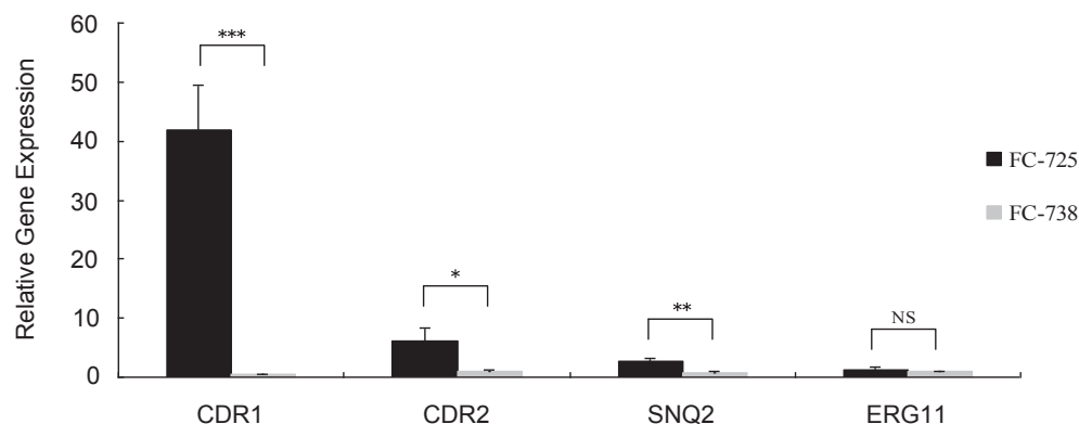
Fig. 3. Expression levels of fluconazole resistance-related genes. The fold changes are determined from the mean normalized expression relative to that of C. glabrata ATCC 90030. FC-725 is a fluconazole-resistant (64 µg/mL) C. glabrata strain. FC-738 is the C. glabrata strain most susceptible to fluconazole (1 µg/mL). All error bars represent the mean ± standard deviation from triplicate tests. NS: not significant, *P < 0.05, **P < 0.01, ***P < 0.001.
