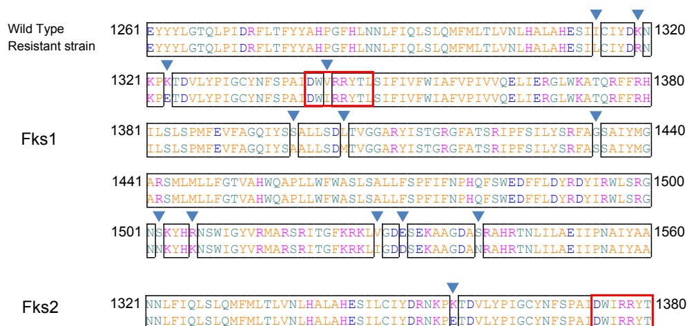
Fig. 2. Alignment of the deduced FKS1 and FKS2 amino acid sequences from C. glabrata CBS138 and micafungin-resistant C. glabrata strain using GENETYX 12.0 (Genetyx Co., Ltd., Tokyo, Japan). The red rectangular boxes indicate FKS hotspot regions. The blue triangles above the amino acid sequences indicate substituted amino acid positions in FKS .
