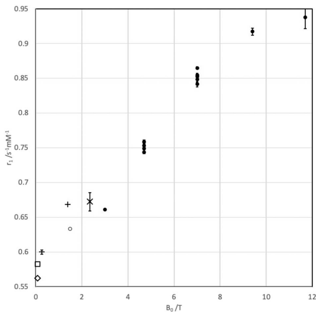
Fig. 2. Plot of [\text{Ni}^{2+}] relaxivities in 2% agarose against field strength. Closed circles: this work, 19.36 \pm 1.20^\circ\text{C} . Open circle: data from initial 1.5 T characterization of the phantom materials (see supplementary material), 21.5^\circ\text{C} . Standard error of fit is shown, although for B_0 between 1.5 T and 7 T the standard errors of between 0.19% and 0.48% are not evident as they are smaller than the size of the symbol. Other symbols: estimated from literature. +, parameter c_1 in [3], 22^\circ\text{C} . —, estimated, with standard error, from Fig. 1 in [9], 22^\circ\text{C} . ×, estimated, with standard error, from Fig. 4 in [15], 20^\circ\text{C} . ◇, □, estimated from Fig. 2 in [16], 19^\circ\text{C} and 22^\circ\text{C} respectively.
