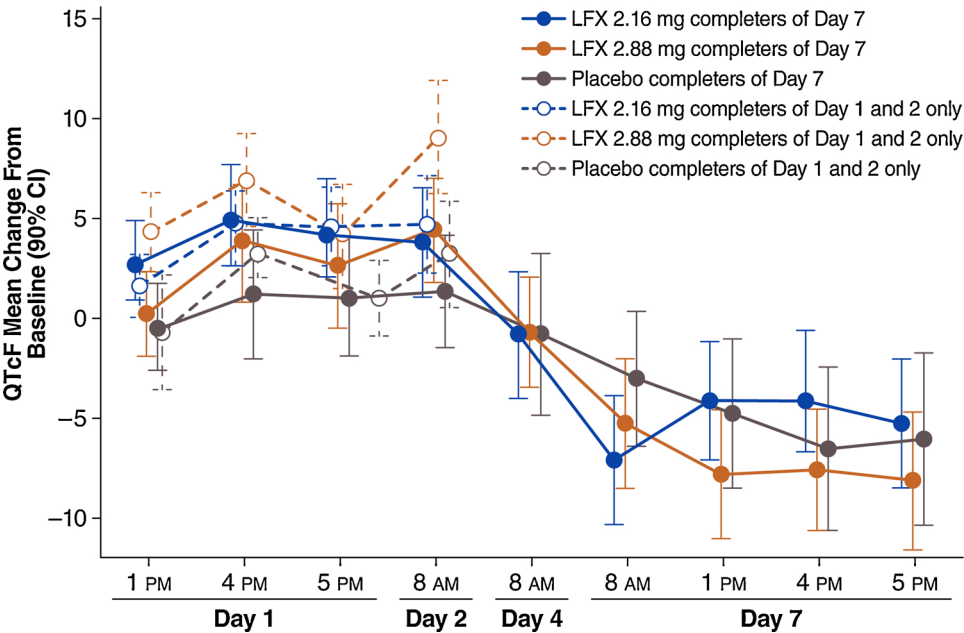
Fig. 4. Change-from-baseline QTcF ( \Delta\text{QTcF} , ms) by completer status. The same pattern of mild QTc prolongation on Day 1 that disappears with continued dosing was seen in subjects with data from all days, i.e., up to and including Day 7, as compared to the full study population (Fig. 2). In subjects with data on Days 1 and 2 only, the effect on \Delta\text{QTcF} was somewhat more pronounced in the lofexidine 2.88 mg group. LFX, lofexidine; QTcF, QT interval corrected, Fridericia formula.
