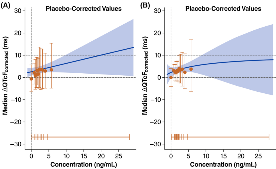
Fig. 3. Predicted QT effect (placebo-corrected \Delta\text{QTcF} , ms) across lofexidine plasma concentrations based on the (A) linear model with baseline and (B) E_{\text{max}} model with baseline. Goodness-of-fit plot with predicted effect on \Delta\text{QTcF} , with 90% confidence intervals (90% CI; black line with grey shaded area). The \Delta\text{QTcF} values are adjusted for the placebo response and correspond to placebo-corrected \Delta\text{QTcF} as used in other analyses. The horizontal bars near the lower edge of the figures show the lofexidine plasma concentration decile breakpoints (hatch marks). The vertical bars and whiskers show the interquartile ranges about the observed median placebo-corrected \Delta\text{QTcF} (solid circles) within each concentration decile. The shaded areas between the two curvilinear lines in each graph show the 90% CI for the \Delta\text{QTcF} as calculated from the two models. Both models predict a small QT effect with increasing lofexidine plasma concentrations. With the linear model, an effect on placebo-corrected \Delta\text{QTcF} larger than 10 ms can be excluded up to lofexidine plasma concentrations of \sim 10 ng/mL.
