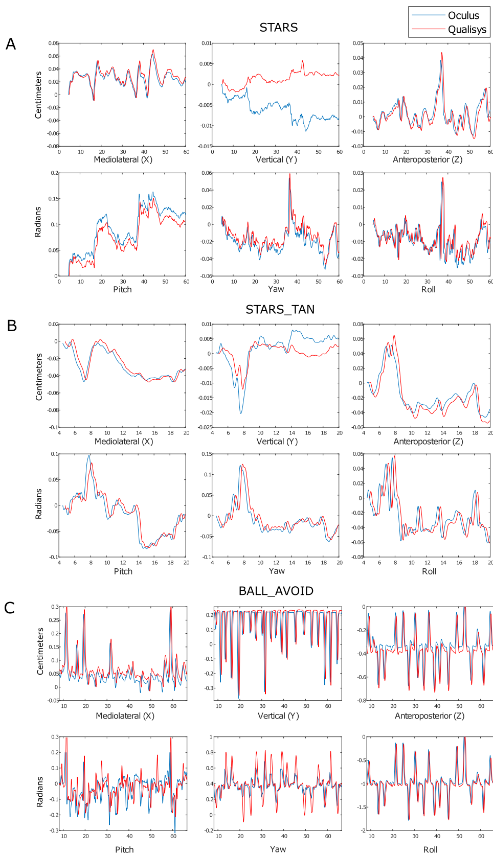
Fig. 3. Head kinematics measured by Oculus Rift (blue) and Qualisys motion capture (red) in 6 degrees of freedom (3 axes of translation and 3 axes of rotation) for (A) A static postural task where the participant watches a 'moving room' with randomly distributed white spheres moving at a frequency of 0.2 Hz and an amplitude of 32 mm (STARS), (B) A similar task where the participant is asked to stand in a tandem leg position (STARS_TAN), and (C) A dynamic task where the participant is required to avoid a ball moving towards them (BALL_AVOID). (For interpretation of the references to colour in this figure legend, the reader is referred to the web version of this article.)
