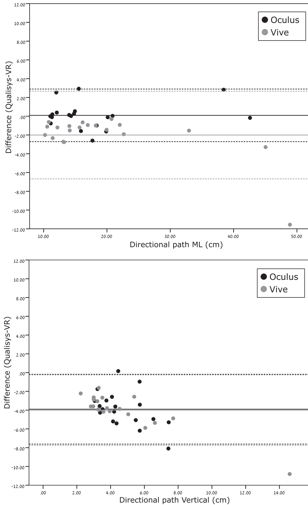
Fig. 4. Examples of Bland and Altman plots demonstrating the bias between Oculus (black) and Vive (grey) with Qualisys motion capture in the STARS task (see text). Solid lines denote the mean bias in directional path (DP) between Oculus/Vive and Qualisys, dashed lines denote 1.96 standard deviations from the mean. The top panel demonstrates bias in mediolateral directional path, while the bottom demonstrates bias in vertical direction, where increased DP values for Oculus and Vive generate a negative bias in both VR systems.
