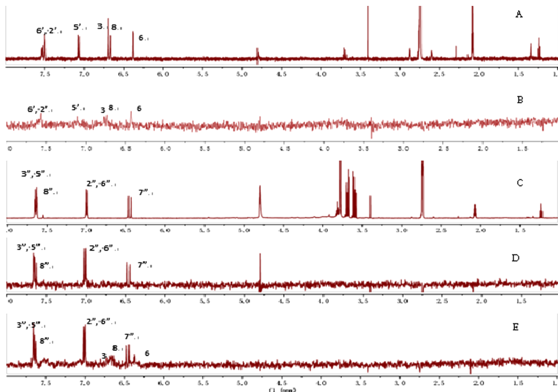
Fig. 2. ^1H NMR and STD-NMR spectra of 1 and 2.
