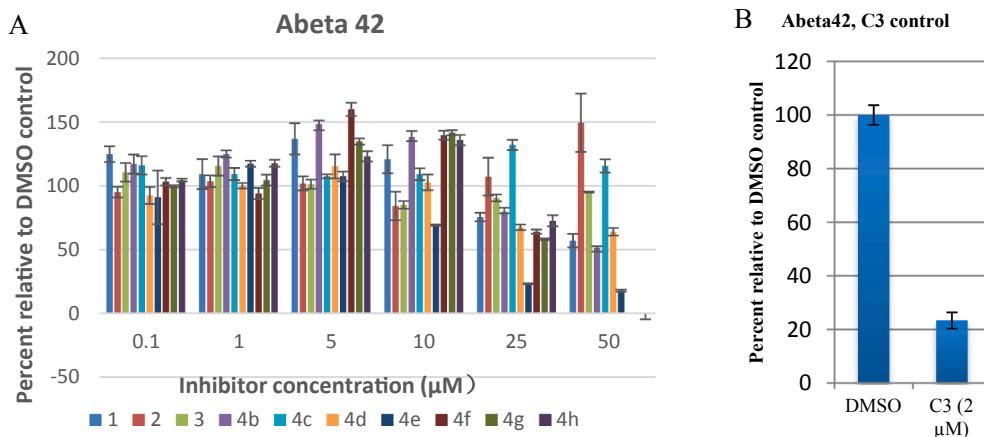
Fig. 4. BACE1 inhibitory activity in cells. (A) The normalized Aβ1-42 level in APP overexpressing HEK293 cells after the treatment of 1 , 2 , 3 , 4b ~ 4h , compared with DMSO (100%). (B) Aβ1-42 level for DMSO and the known inhibitor C3 [20].
