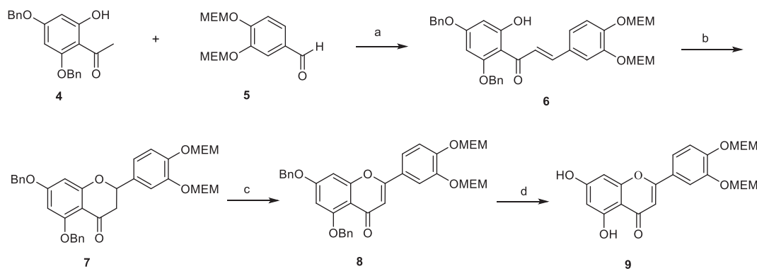
Scheme 1. Synthesis of intermediate 9 . Reagents and conditions: a. 20% KOH aq. ethanol, room temperature, 54%; b. NaOAc, H 2 O, ethanol, reflux, 46%; c. I 2 , pyridine, 100 °C, 69%; d. H 2 , Pd/C, EtOAc, room temperature, 85%.
