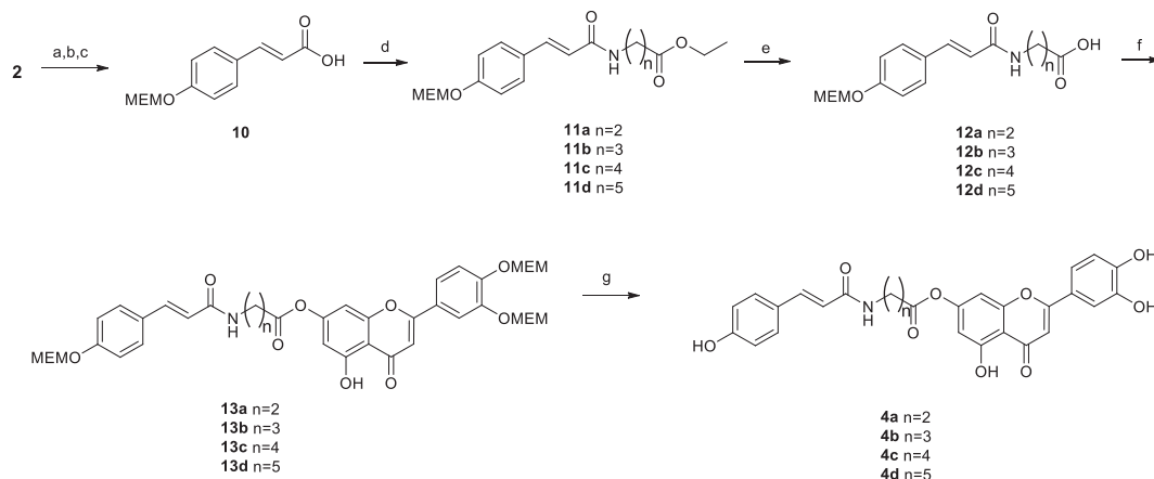
Scheme 2. Synthesis of conjugates 4a-d . Reagents and conditions: a. EtOH, conc. H 2 SO 4 , 95%. b. MEMCl, DIEA, DCM, rt, 91%. c. LiOH, EtOH, THF, H 2 O, 95%. d. (i) SOCl 2 , MeOH, reflux, (ii) 1-(3-DiMethylaminopropyl)-3-ethylcarbodiimide hydrochloride (EDCI), dimethylaminopyridine (DMAP), Et 3 N, CH 2 Cl 2 , r.t., 56%-83%. e. LiOH, EtOH, tetrahydrofuran (THF), H 2 O, 84%-98%. f. 9 , EDCI, DMAP, Et 3 N, CH 2 Cl 2 , 40 °C, 30%-57%. g. Iodotrimethylsilane (TMSI), CH 3 CN, -20 °C, 67%-88%.
