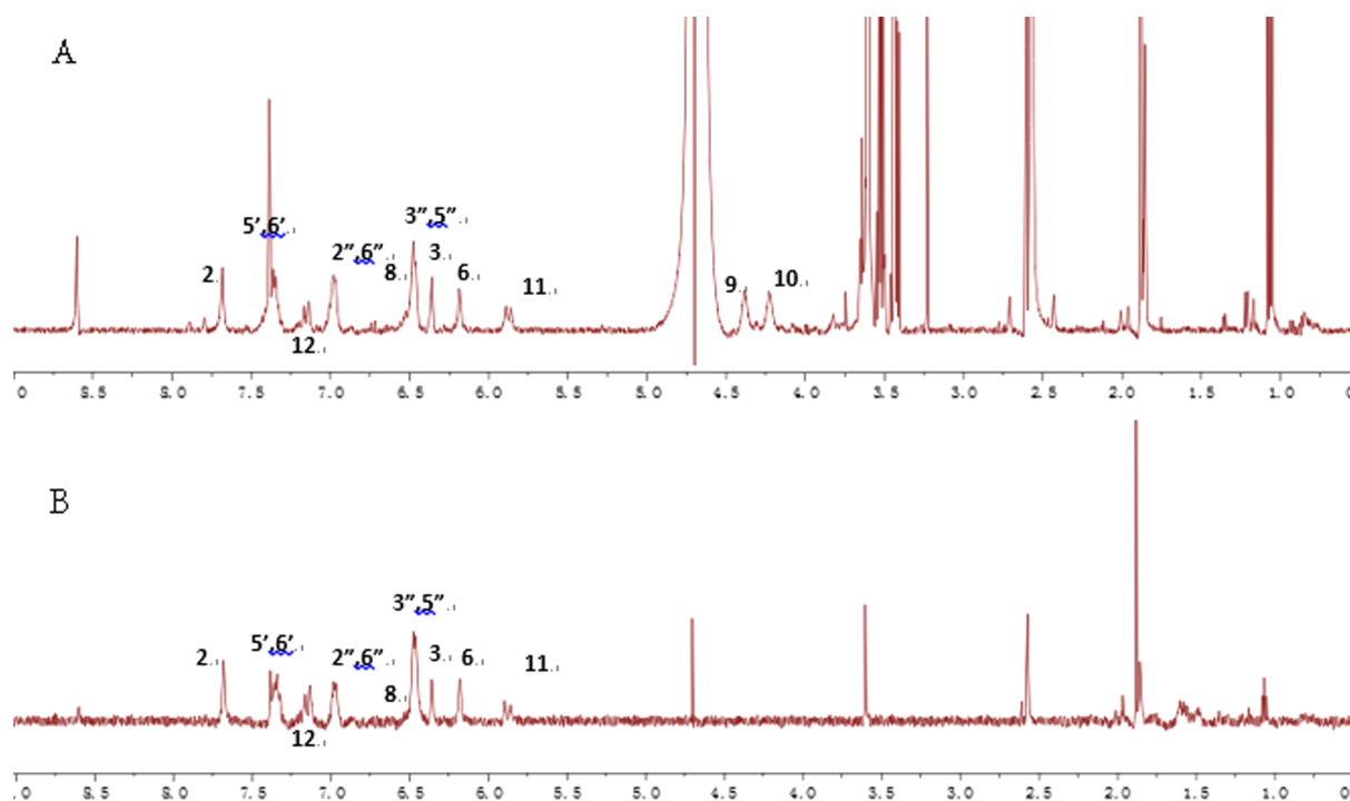
Fig. 6. NMR and STD-NMR spectra of 4j. (A) ^1\text{H} NMR of 4j (2 mM) with BACE1 (10 \mu\text{M} ); (B) STD-NMR of 4j (2 mM) with BACE1 (10 \mu\text{M} ).
