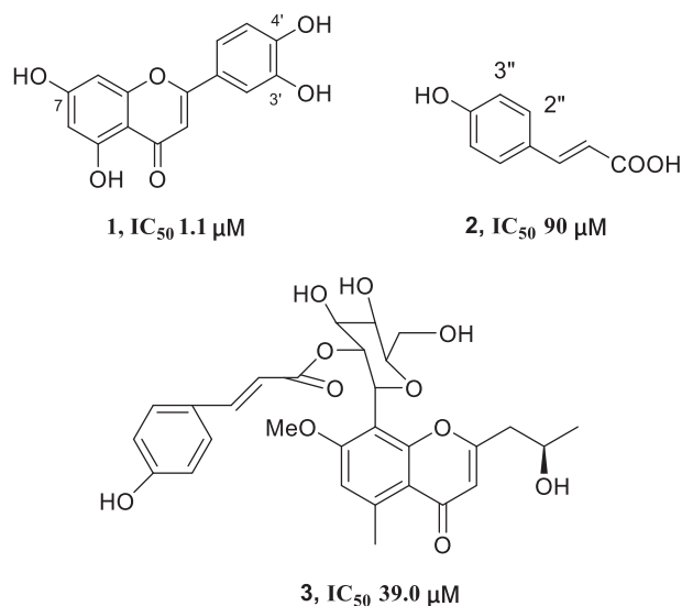
Fig. 1. Structures of BACE1 inhibitory natural products and their IC_{50} inhibitory BACE1 in references.
