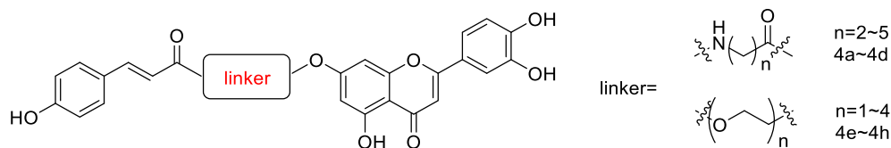
Fig. 3. The design of conjugates 4.
