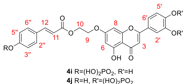
Fig. 5. The structures of phosphates 4i and 4j .
