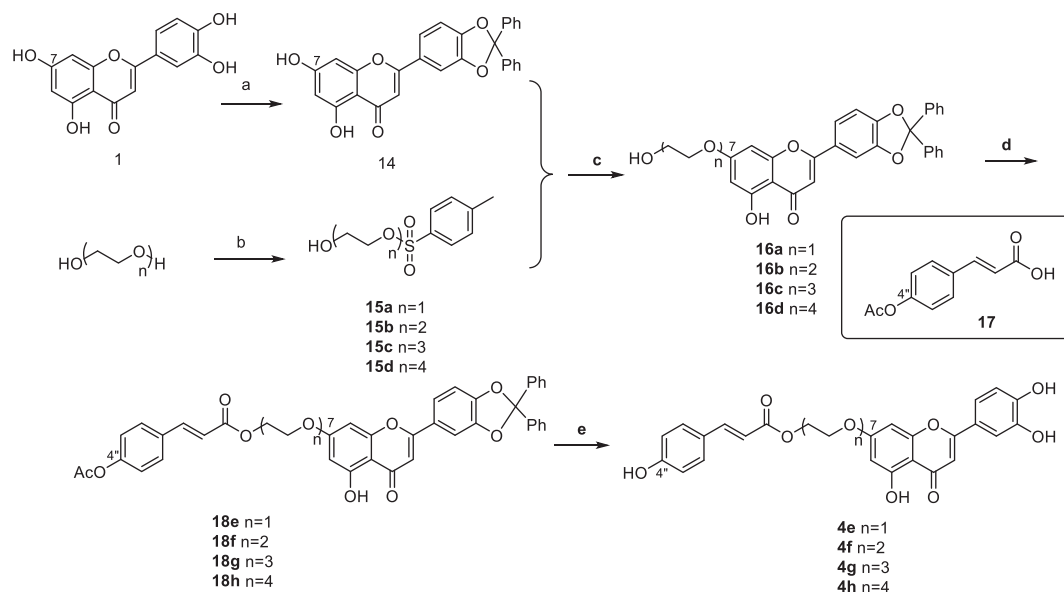
Scheme 3. Synthesis of conjugates 4e-h . Reagents and conditions: a. dichlorodiphenylmethane, diphenyl ether, 165 °C, 70%. b. TsCl, Et 3 N, DCM, 40 °C, 21–23%. c. K 2 CO 3 , CH 3 CN, reflux, 46%–79%. d. 17 , EDCI, DMAP, Et 3 N, THF, 40 °C, 34%–60%. e. aq. 38% HCl in AcOH (v/v 1:15), r.t., 26–80%.
