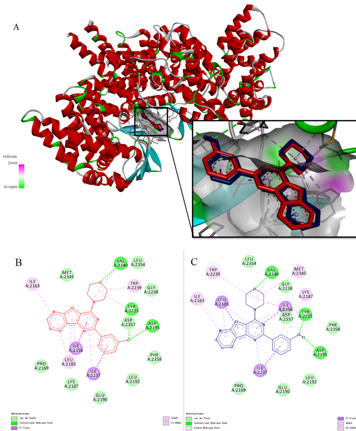
Fig. 6. A: Stacking map of re-docked PI-103 (blue) and the original ligand (red); B: the binding mode of original ligand (red) with mTOR (PDB:4jt6); C: the binding mode of re-docked PI-103 (blue) with mTOR (PDB:4jt6).
