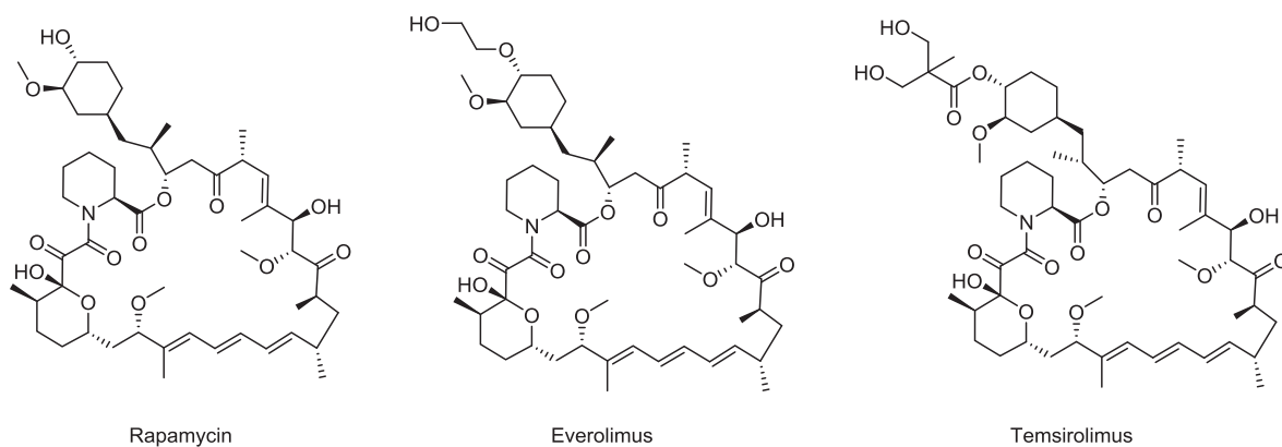
Fig. 1. Chemical structures of Rapamycin and Rapamycin analogs.
