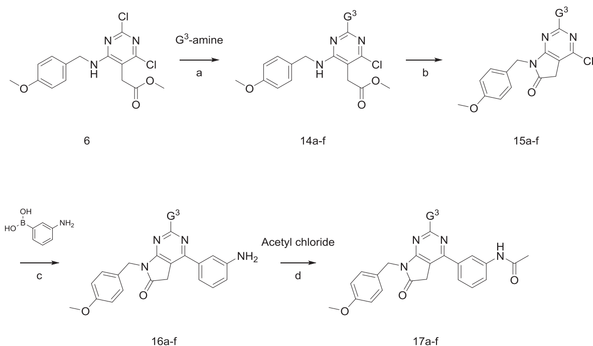
Scheme 4. Reagents and conditions: (a) 4-DMAP, DMF; (b) TsOH, Toluene; (c) (dppf) 2 PdCl 2 , Na 2 CO 3 , Dioxane/H 2 O; (d) DIPEA, DCM.
