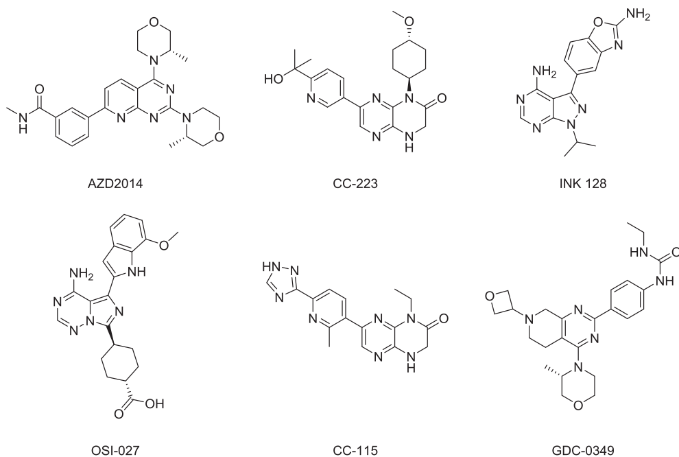
Fig. 2. Chemical structures of mTORC1/mTORC2 dual-target inhibitors.
