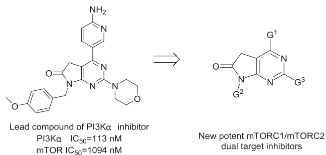
Fig. 3. Optimization design of 5,7-dihydro-6H-pyrrolo[2,3-d]pyrimidin-6-one derivatives.
