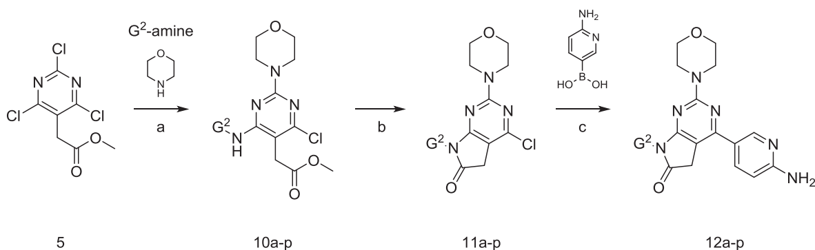
Scheme 2. Reagents and conditions: (a) I DIPEA, DMF, II 4-DMAP, DMF; (b) TsOH, Toluene; (c) (dppf) 2 PdCl 2 , Na 2 CO 3 , Dioxane/H 2 O.
