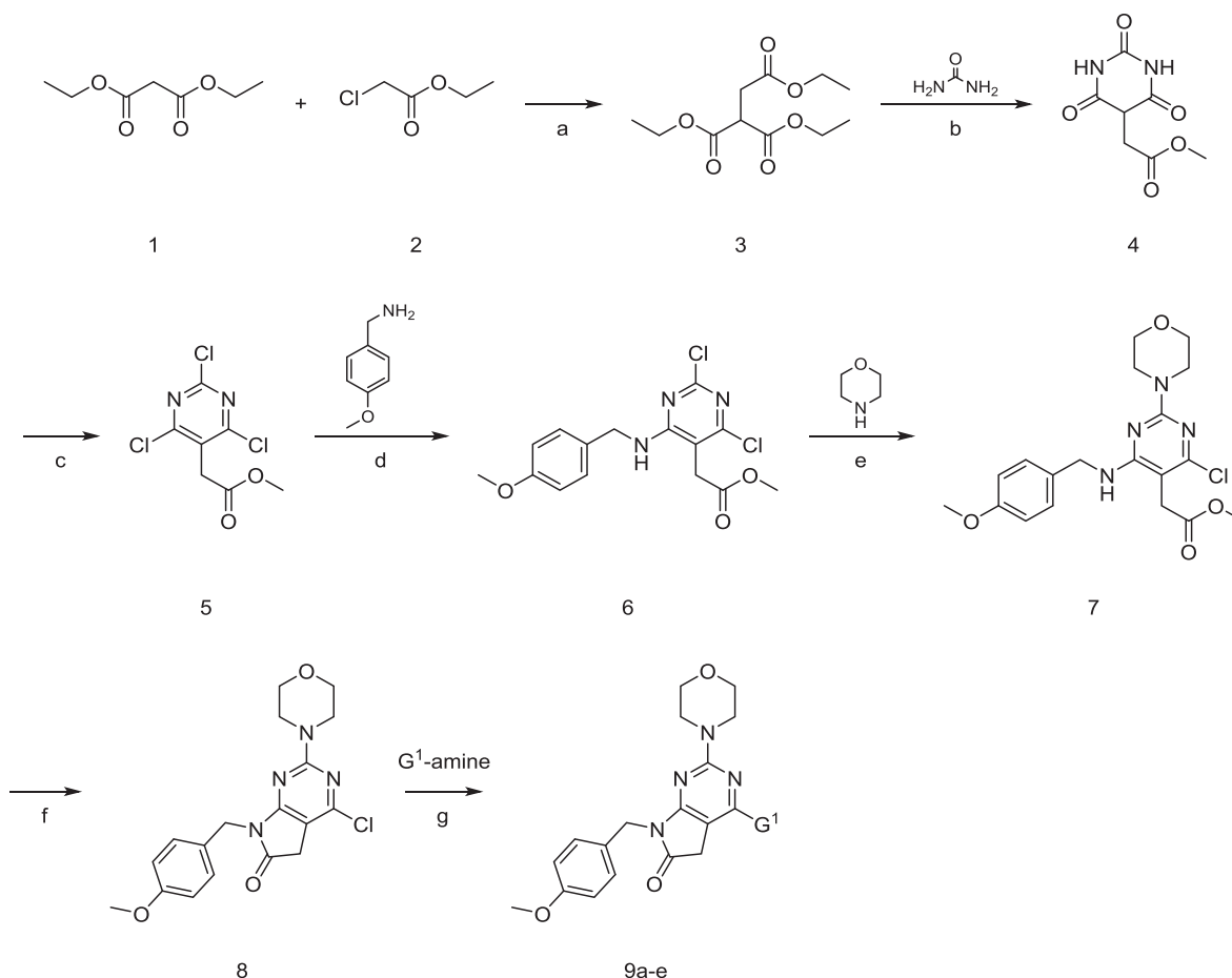
Scheme 1. Reagents and conditions: (a) EtONa, EtOH; (b) MeONa, MeOH; (c) DIPEA, POCl 3 ; (d) DIPEA, DMF; (e) 4-DMAP, DMF; (f) TsOH, Toluene; (g) DIPEA, DMA.
