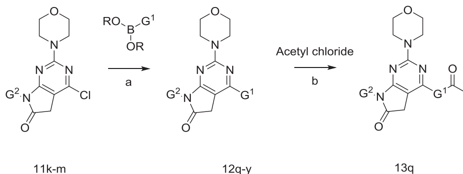
Scheme 3. Reagents and conditions: (a) (dppf) 2 PdCl 2 , Na 2 CO 3 , Dioxane/H 2 O; (b), DIPEA, DCM.
