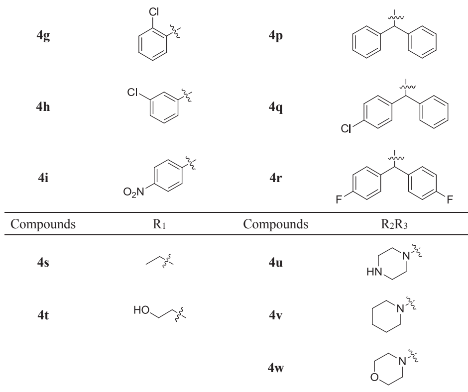
Scheme 1. (continued)
