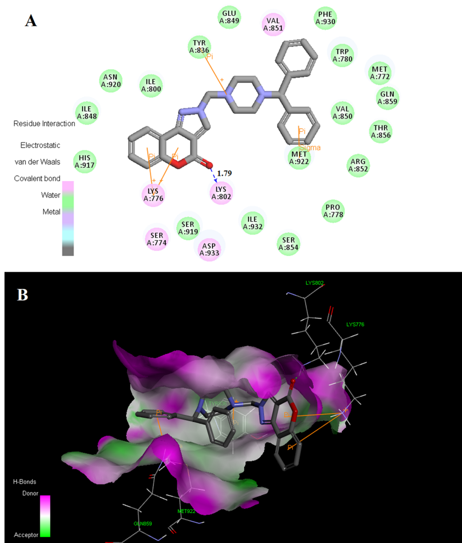
Fig. 4. (A) 2D molecular docking model of compound 4p with 3HHM (PI3Kα H1047R mutant). (B) 3D conformation position of the compound 4p in the binding pocket.
