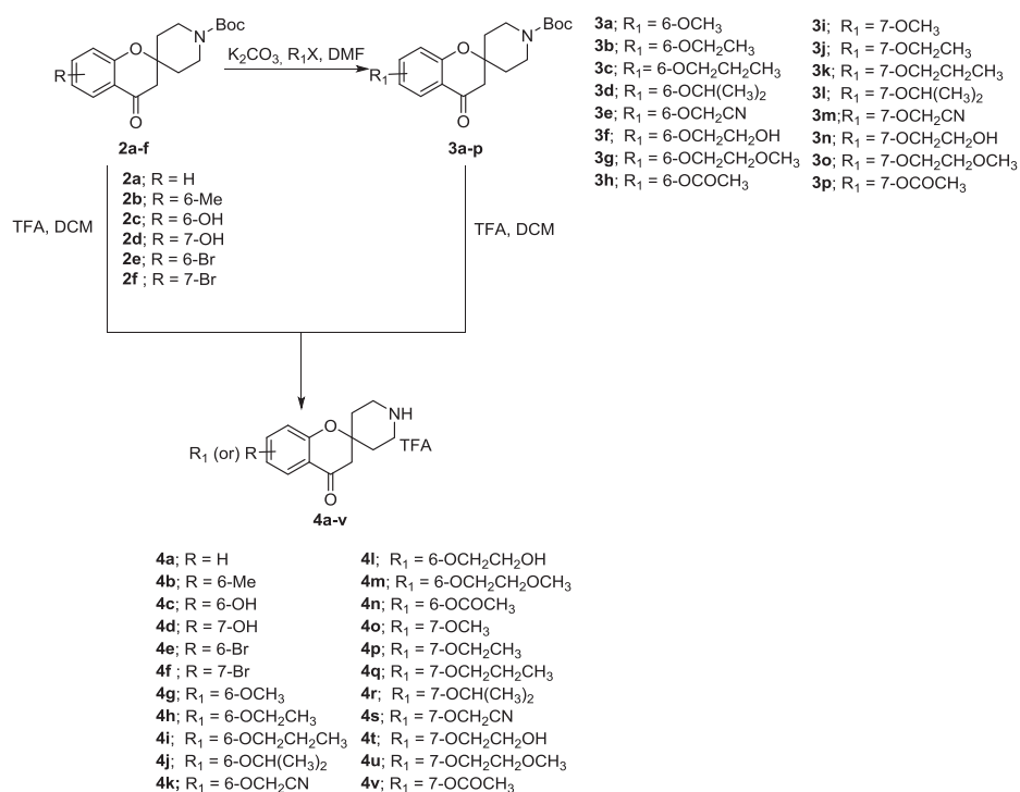
Scheme 3. General procedure to obtain spiroamines 4a-v.
