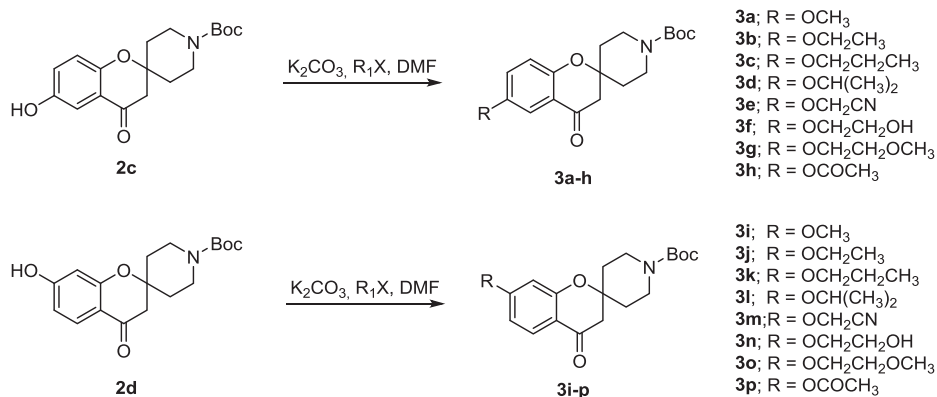
Scheme 2. General procedure to synthesize compounds 3a-p.
