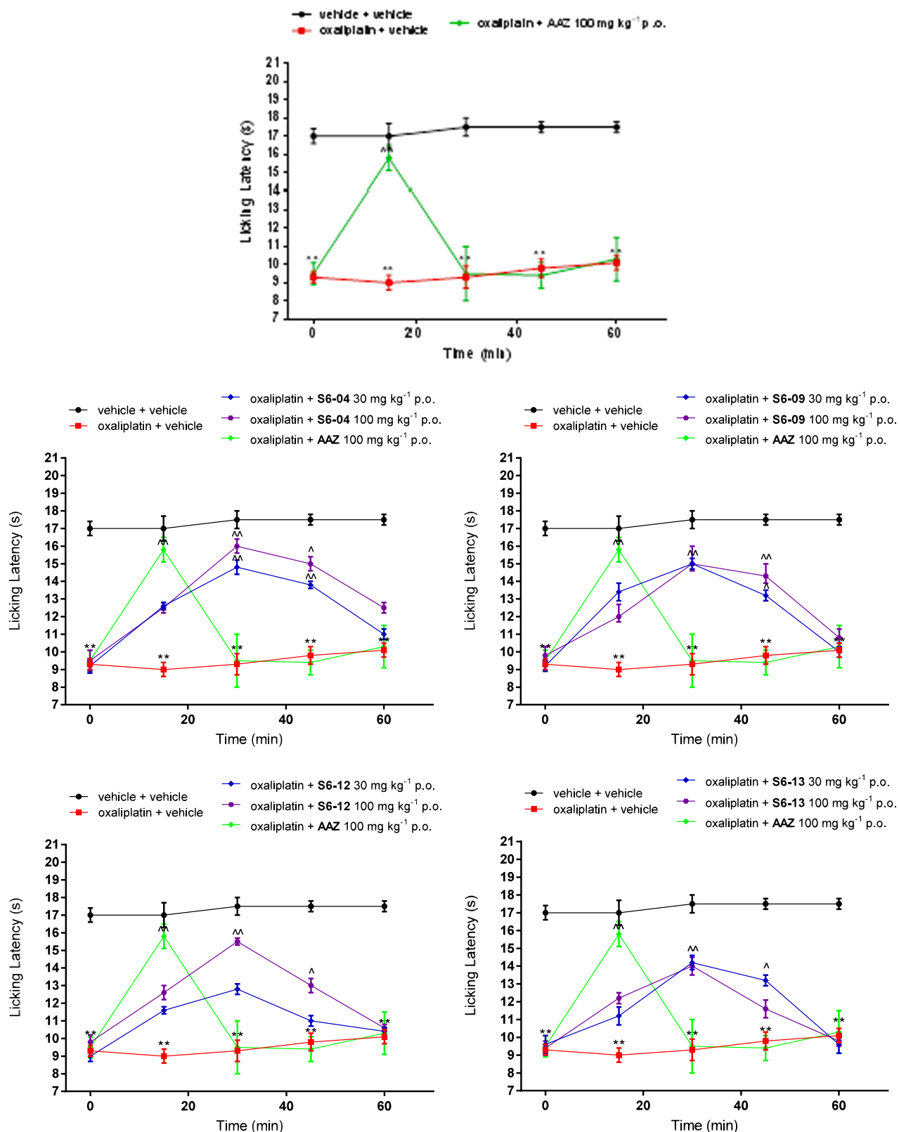
Fig. 1. Effect of acute administration of carbonic anhydrase inhibitors 6d , 6i , 6l and 6m and AAZ on oxaliplatin induced neuropathic pain in the mouse Cold plate test **P < 0.01 vs vehicle + vehicle treated animals; *P < 0.05 and ~P < 0.01 vs oxaliplatin + vehicle treated animals. Each value represents the mean \pm S.E.M. of 10 mice performed in 2 different experimental sets.
