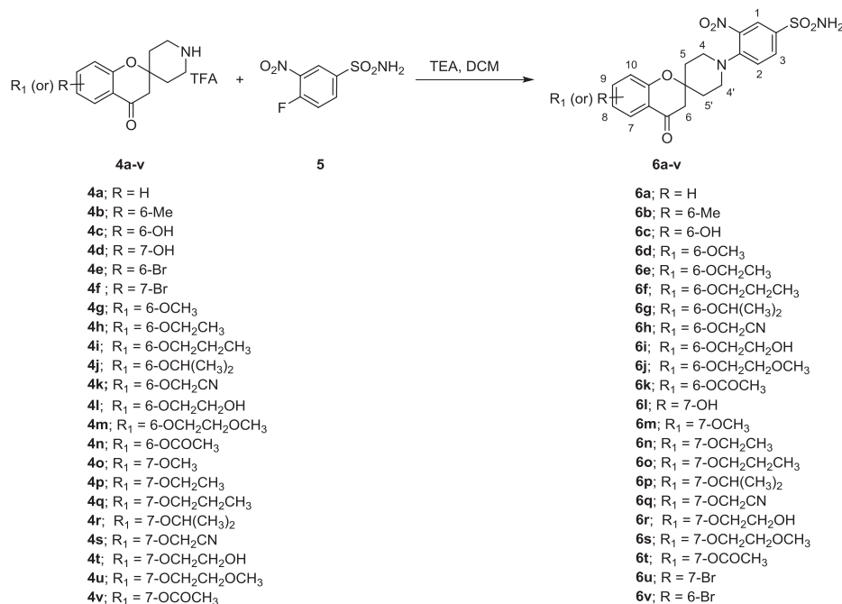
Scheme 4. General procedure to obtain 3-nitrobenzenesulfonamide derivatives 6a-v .
