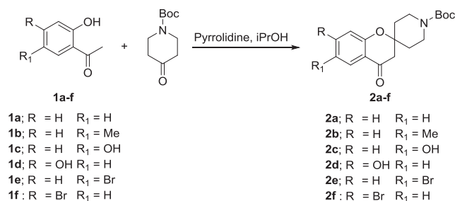
Scheme 1. General procedure to obtain derivatives 2a-f.
