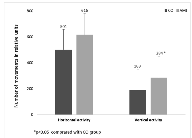
Fig. 2. Effects of A. melanocarpa fruit juice supplementation on activity cage test in rats.
