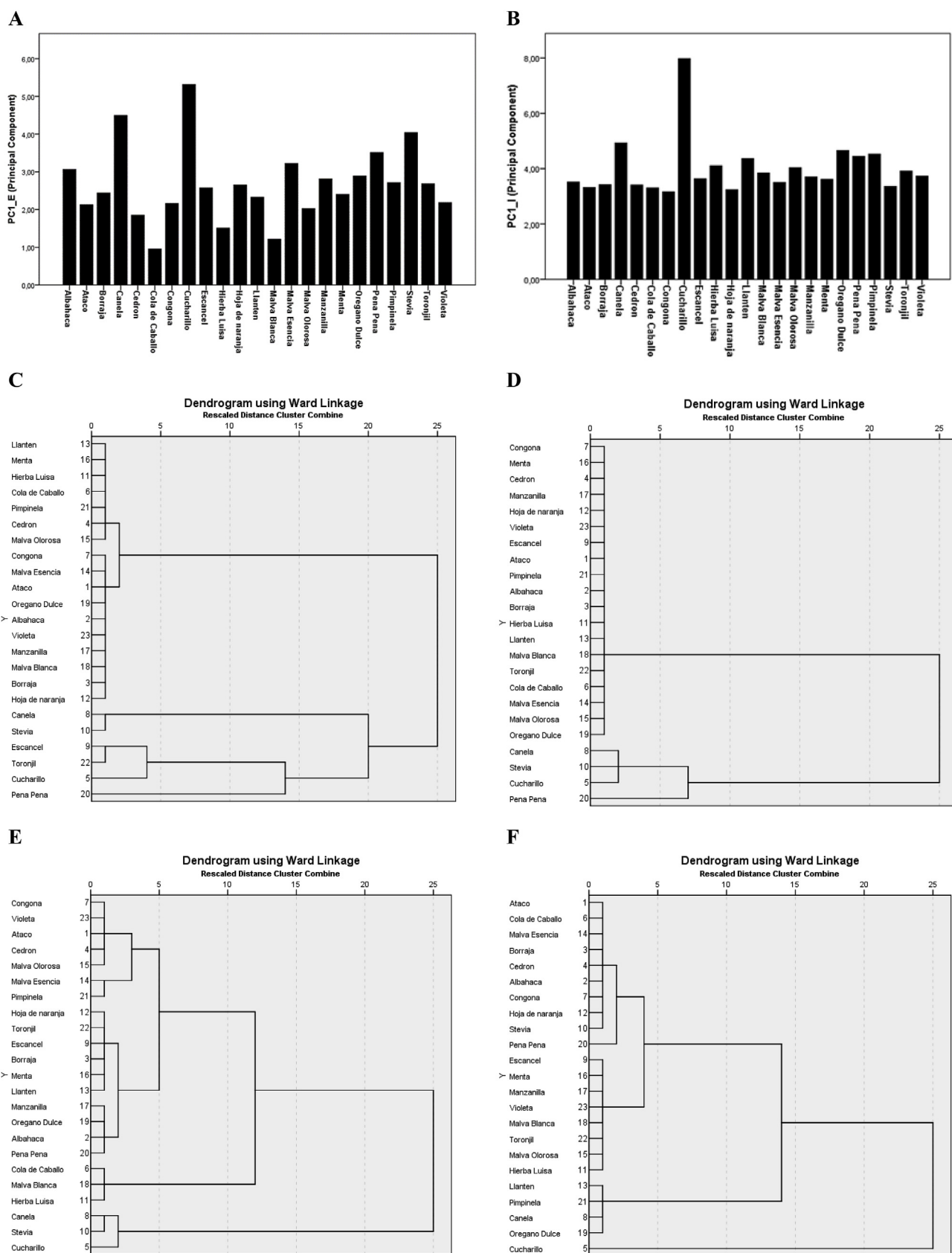
Fig. 2. Histograms obtained from the factorial analysis considering the variables FRAP and DPPH using varimax rotation for the hydroalcoholic extract (A) and infusion (B) of each plant conform the horchata drink. Dendrograms created using Ward's method considering the phytochemical composition for the hydroalcoholic extract (C) and infusion (D), and the antioxidant capacity (DPPH and FRAP) for the hydroalcoholic extract (E) and infusion (F).
