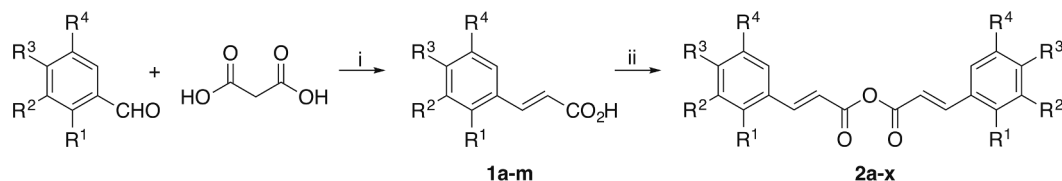
Scheme 1. . Synthesis of cinnamic acid derivatives and the appropriate anhydrides: (i): piperidine, pyridine, reflux 120 °C, 4 h; (ii): (1) oxalyl chloride, CH 2 Cl 2 , 0 °C → 25 °C, 2 h (2) pyridine, toluene, 25 °C, overnight.
