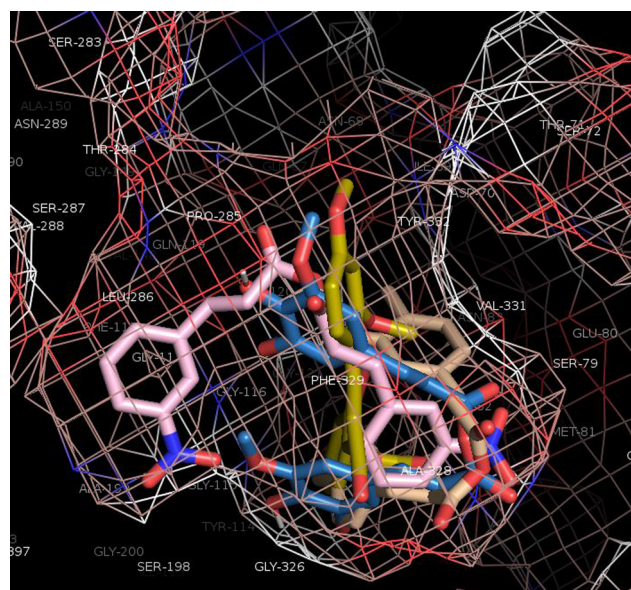
Fig. 2. Compounds 1a-1m (left) and 2a-2x (right) inside the AChE active site pocket.
