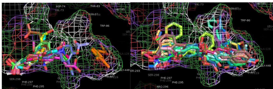
Fig. 2. Compounds 1a-1m (left) and 2a-2x (right) inside the AChE active site pocket.
