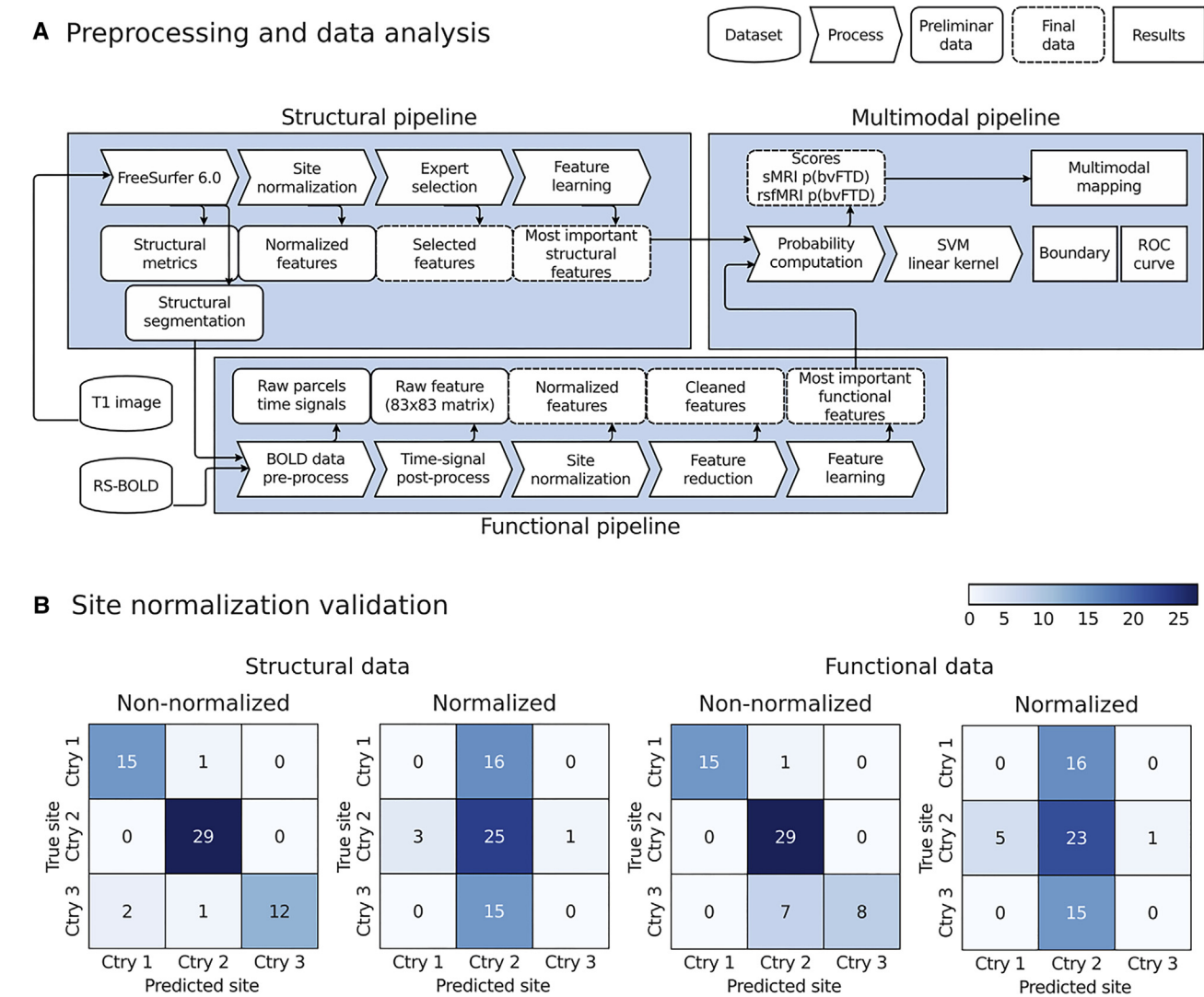
Fig. 1. Preprocessing, data analysis, and site normalization. (A) Main overview of the processing framework used for the multimodal integration of structural and functional information using machine learning techniques. p(bvFTD) refers to the probability of being classified as a behavioral variant frontotemporal dementia (bvFTD) patient, SVM refers to support vector machine classifier, ROC to receiver operating characteristic, RS to resting state, BOLD to blood oxygen level dependent, sMRI to structural MRI, and rsfMRI to resting-state functional MRI. (B) Confusion matrix before and after the site normalization process for both structural data (left) and functional data (right).
