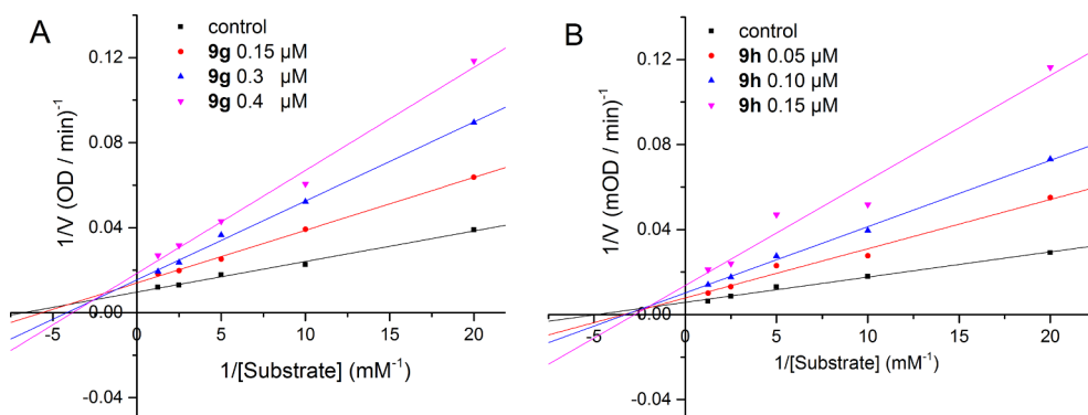
Fig. 3. Lineweaver-Burk plots of BChE inhibition of 9g (A) and 9h (B).
