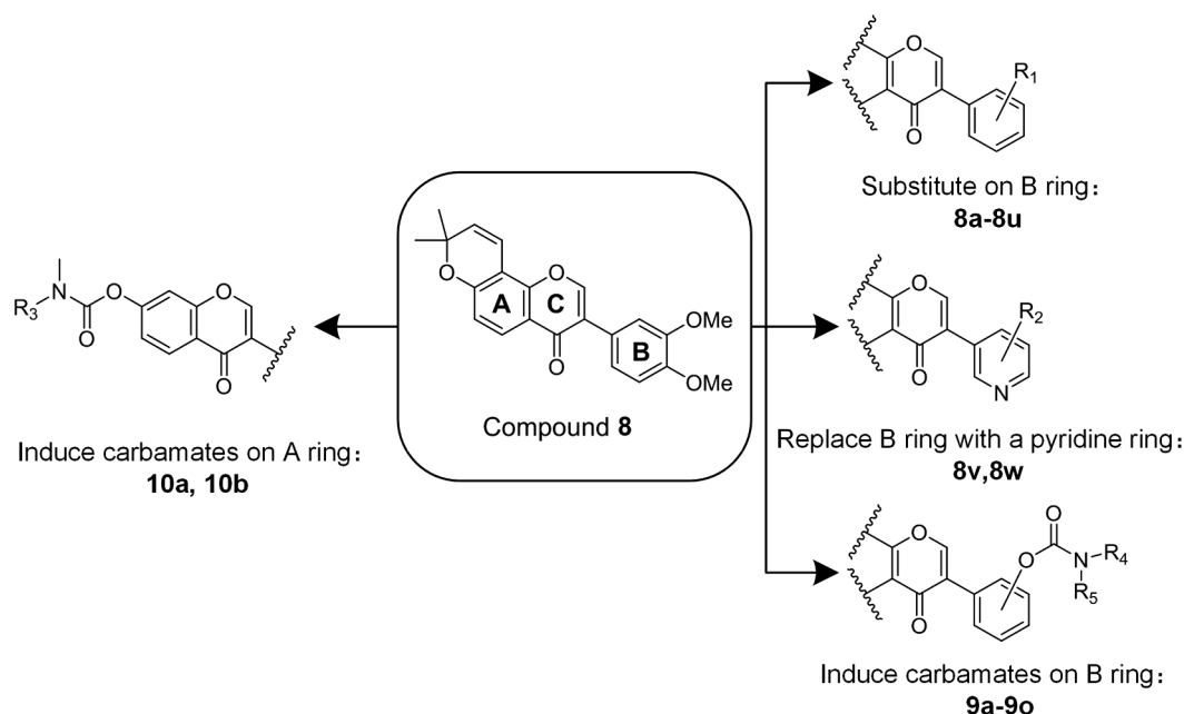
Fig. 1. Design strategy carried out starting from compound 8.
