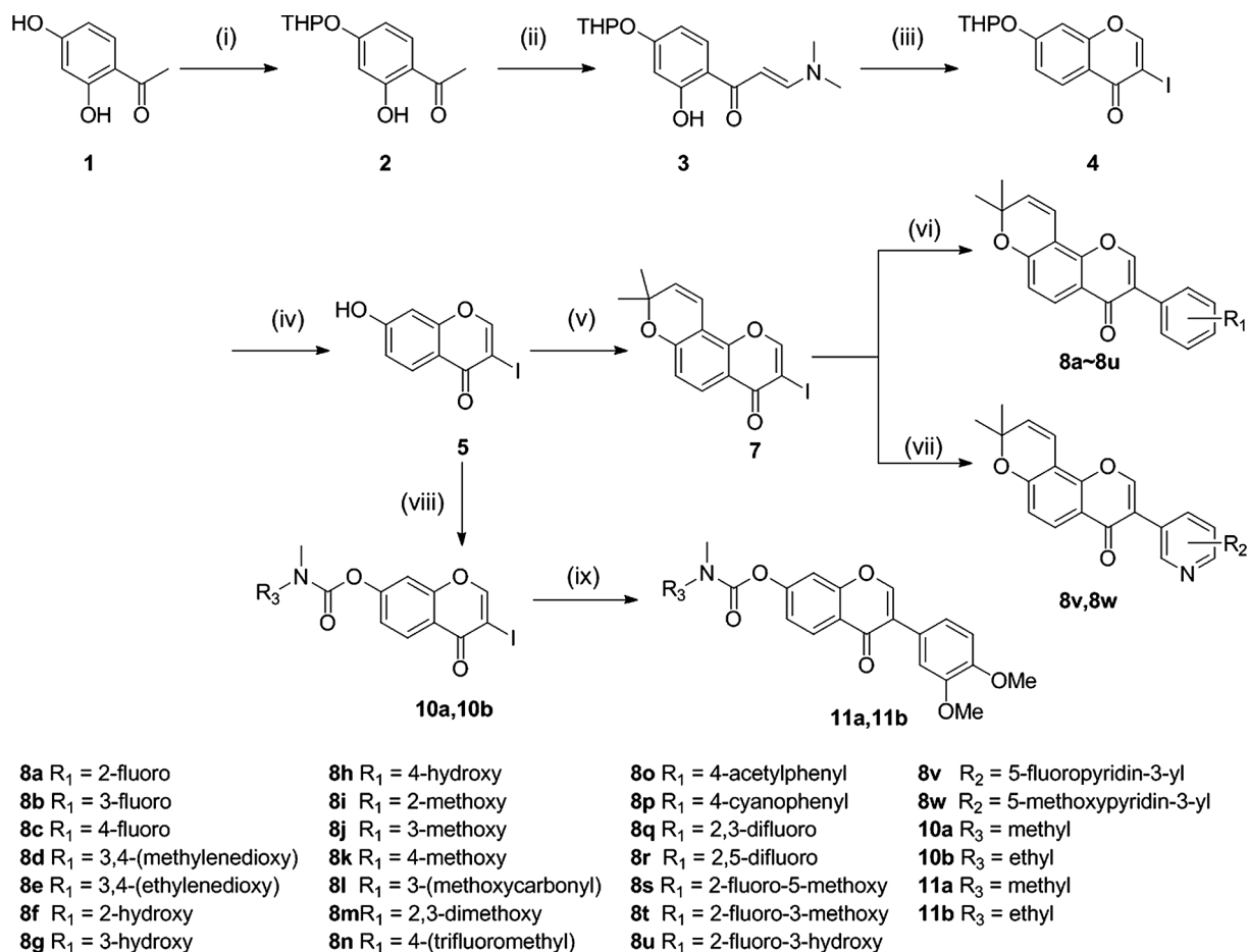
Scheme 1. Synthesis of compounds 8a-8w and 11a-11b . Reagents and conditions: (i) DHP, PPTS, CH 2 Cl 2 , rt, 4 h; (ii) DMF-DMA, 95 °C, 3 h; (iii) I 2 , pyridine, CHCl 3 , rt, 12 h (74.7% for three steps); (iv) pTsOH, CH 3 OH, THF, 60 °C, 1 h; (v) 1,1-diethoxy-3-methyl-2-butene, 3-picoline, xylene, reflux, 24 h; (vi) ArB(OH) 2 , 10% Pd/C, Na 2 CO 3 , H 2 O, DME, 45 °C, 1 h; (vii) heteroaryl boronic acids, Pd[P(C 6 H 5 ) 3 ] 4 , Na 2 CO 3 , THF, H 2 O, 60 °C, 6 h; (viii) acyl chloride, K 2 CO 3 , DMF, CH 3 CN, 95 °C, 3 h; (ix) ArB(OH) 2 , 10% Pd/C, Na 2 CO 3 , H 2 O, DME, 45 °C, 1 h;
