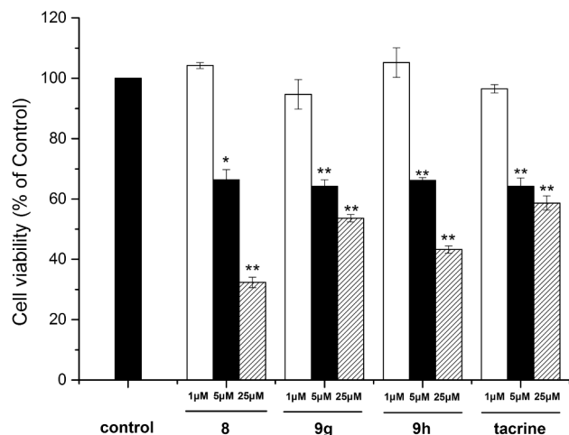
Fig. 5. In vitro cytotoxicity of compounds 8 , 9g and 9h on PC12 cell line. Data were expressed as mean \pm SD (n = 3). * p < 0.05, ** p < 0.01 vs Ctrl.
