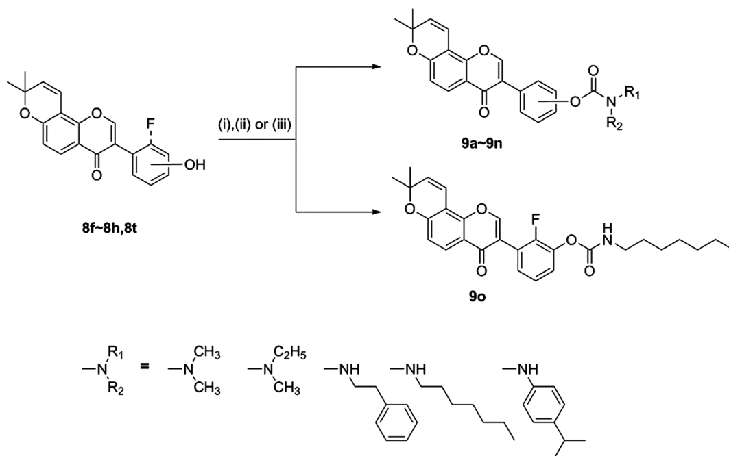
Scheme 2. Synthesis of compounds 9a-9o . Reagents and conditions: (i) acyl chloride, K 2 CO 3 , DMF, CH 3 CN, 95 °C, 3 h; (ii) isocyanate, NEt 3 , CH 2 Cl 2 , rt, 6 h; (iii) acyl chloride, K 2 CO 3 , CH 3 CN, rt, 24 h.
