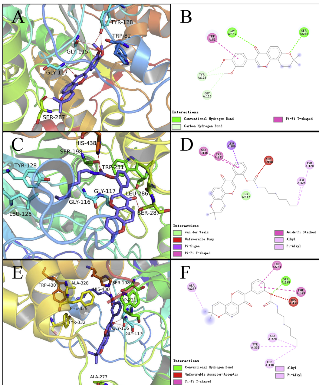
Fig. 4. Binding mode of 8 (A and B), 9g (C and D) and 9h (E and F) in the BChE active site. Figures (B, D and F) were made by Discovery Studio 2016 Client software; Figures (A, C and E) were created with PyMol 1.8.2.0.
