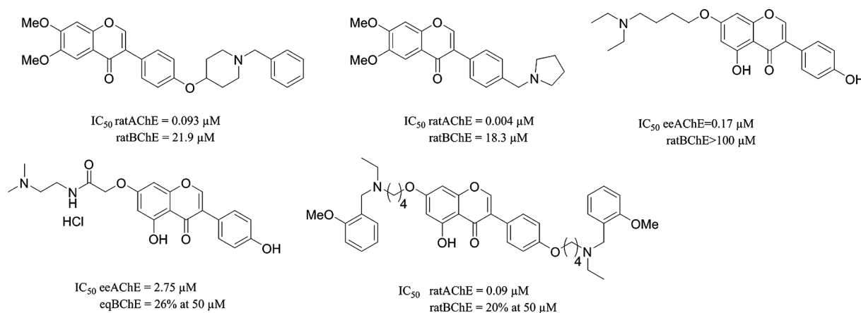
Fig. 2. Isoflavone-based structures which have been investigated as ChE inhibitors.
