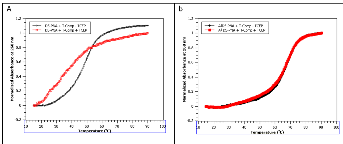
Fig. 3. Thermal melting curves of (a) DS-PNA:T-Comp with and without TCEP and (b) A/DS-PNA:T-Comp under the same conditions. Each strand was 1 \mu M.
