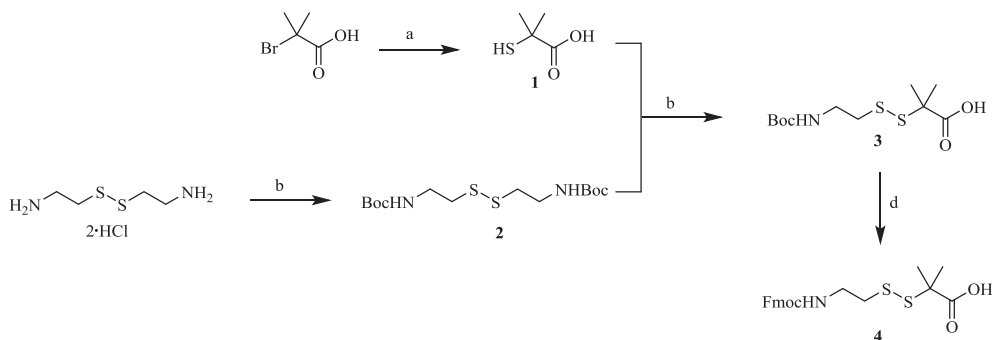
Scheme 1. Reaction scheme for synthesized compound 4. a. thiourea, NaOH, H 2 O, 80 °C, 23% b. Di- tert -butyl-dicarbamate, dioxane, 2 M NaOH, 54% c. 30% H 2 O 2 , NaOH, H 2 O, 49% d. (1) TFA, m-cresol; (2) DIPEA, Fmoc-Cl, DCM, 53%.
