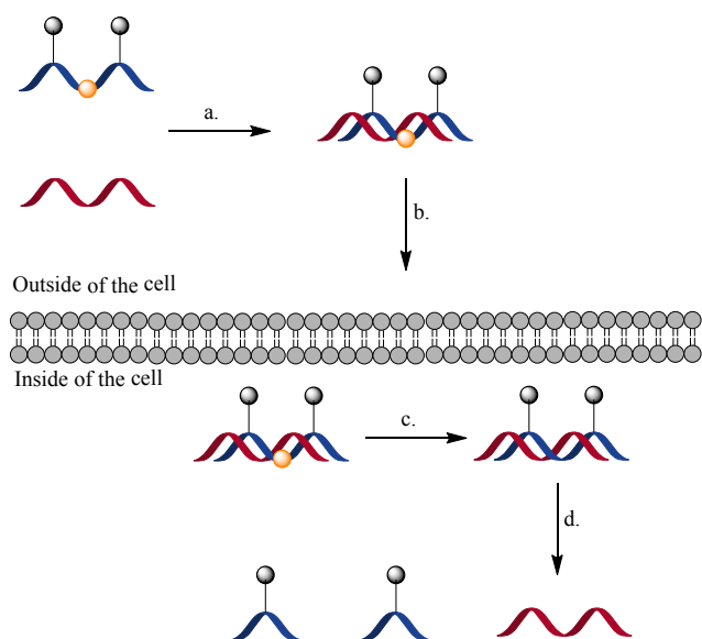
Fig. 1. Conceptual design of a temporary PNA containing a biologically susceptible disulfide bond strand that will assist with the delivery of an antigene or antisense strand to the cytoplasm of a cell. a. Duplex formation of antisense PNA (red) and a temporary PNA (blue) containing a disulfide bond (orange circle) in the backbone and cell penetrating peptides, endosomal escape and/or localization factors (black circles). b. Cellular entry mediated by the temporary strand. c. Reduction of the disulfide bond by endogenous reagents (glutathione). d. Release of a pristine antisense PNA.
