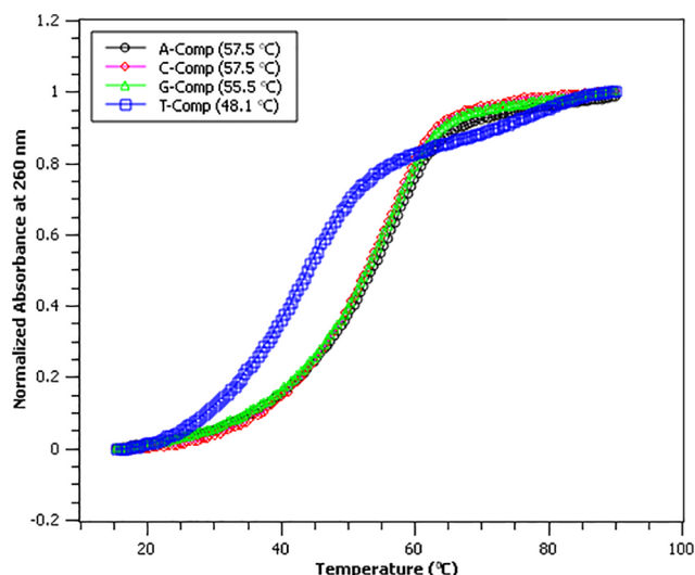
Fig. 2. Thermal denaturation studies of (a) DS-PNA with complementary strands having A, T, G or C opposite the disulfide monomer. Inset shows the T_m of all duplexes. Each strand was 1 \mu M.
