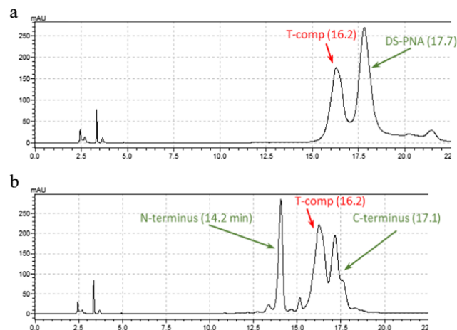
Fig. 4. Chromatograms of DS-PNA/T-Comp. Annealed samples a. before and b. after treatment with TCEP. Peaks are identified based on MS and retention times in minutes are in parenthesis.
