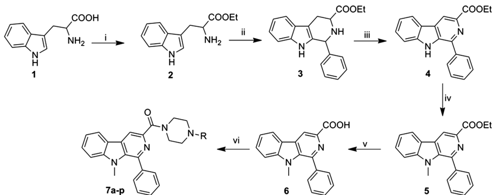
Scheme 1. Reagents and conditions: (i) thionylchloride, ethanol, reflux, 30 min, 76%; (ii) benzaldehyde, trifluoroacetic acid, DCM, rt, 3 h, 82%; (iii) \text{KMnO}_4 , THF, rt, 24 h, 68%; (iv) methyl iodide, KOH, DMSO, rt, 30 min, 72%; (v) 50% aq. NaOH, reflux, 30 min, 78%; (vi) EDCI, HOBt, THF, piperazines, 0 °C–rt 6 h, 62–82%.
