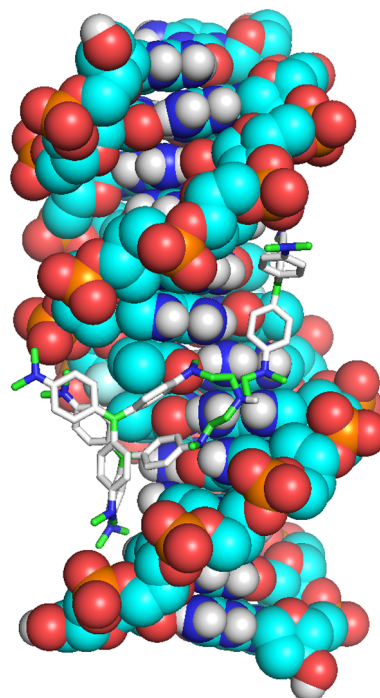
Fig. 7. Model for the binding of ligand 1e in the major groove of the Drew-Dickerson dodecamer (5'-CGCGAATTCGCG-3').
