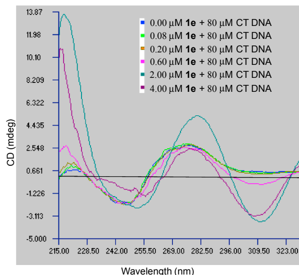
Fig. 6. The 220–310 nm region of the CD spectrum of solutions of CT DNA (80 \mu\text{M} ) in the absence (blue line) and presence of various concentrations of 1e : blue line 0.0 \mu\text{M} 1e , light green line, 0.08 \mu\text{M} 1e ; orange line, 0.20 \mu\text{M} 1e ; light red line, 0.06 \mu\text{M} 1e ; dark green line 2.00 \mu\text{M} 1e ; purple line: 4.00 \mu\text{M} 1e .
