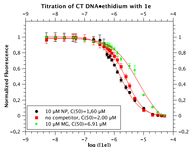
Fig. 4. Binding isotherms for the titration of CT DNA (10 \mu M) and ethidium (10 \mu M) with 1e (10 mM Tris-EDTA, 10 mM NaCl, pH = 5.48) in the absence of competitor (red squares) or in the presence of netropsin (black circles) or methyl green (green diamonds). Black circles: 10 \mu M netropsin, K_a = 13.1 \pm 1.4 \times 10^7 M ^{-1} ; red squares: no competitor, K_a = 10.5 \pm 0.6 \times 10^7 M ^{-1} ; green diamonds: 10 \mu M methyl green, K_a = 3.04 \pm 0.46 \times 10^7 M ^{-1} .
