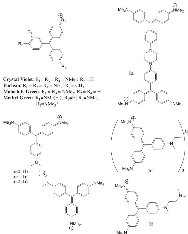
Fig. 1. Structures of cationic dyes and synthetic derivatives 1a–1f .
