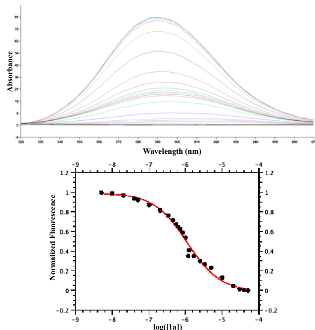
Fig. 2. Displacement of ethidium bromide from CT DNA by 1a .
