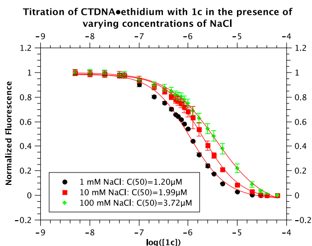
Fig. 3. Titration of CT DNA (10 \mu M) and ethidium (10 \mu M) with 1c : 0.005, 0.01, 0.02, 0.04, 0.05, 0.1, 0.2, 0.33, 0.45, 0.56, 0.63, 0.71, 0.83, 1.00, 1.25, 1.67, 2.50, 3.30, 5.0, 10.0, 20.0, 30.0, 40.0, 50.0 \mu M.
