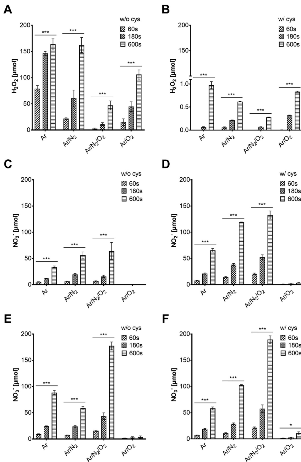
Fig. 2. Deposition of H 2 O 2 (A), NO 2 - (C) and NO 3 - (E) in water or water with 2 mM cysteine (corresponding subfigures B, D, F) (kINPen09, 3 slm Ar + 1% molecular gas admix).
